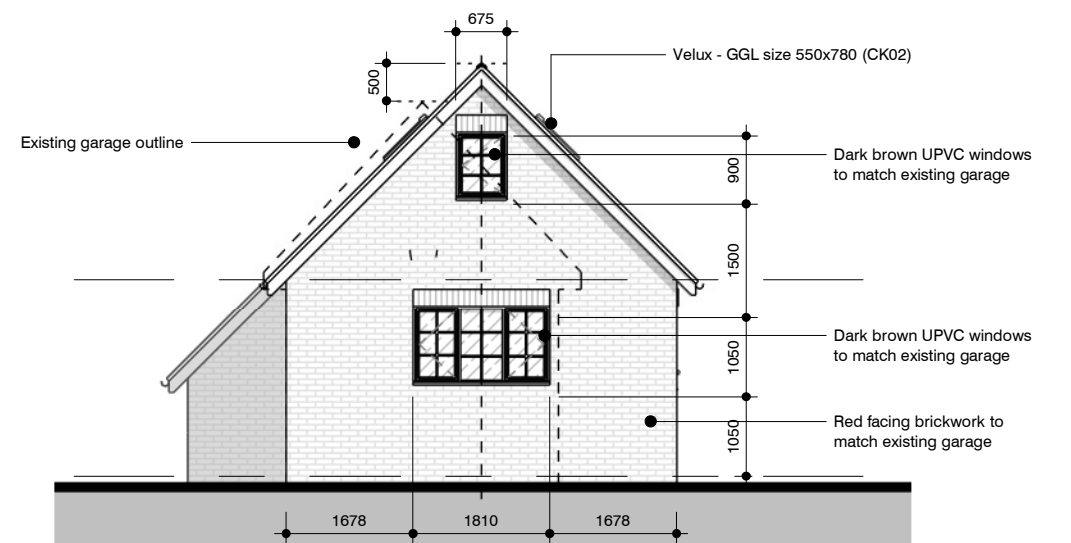
3 North Elevation 1 : 100 @A3
