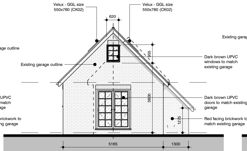
2 South Elevation 1 : 100 @A3
