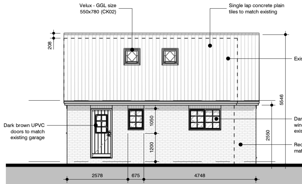
1 East Elevation 1 : 100 @A3
