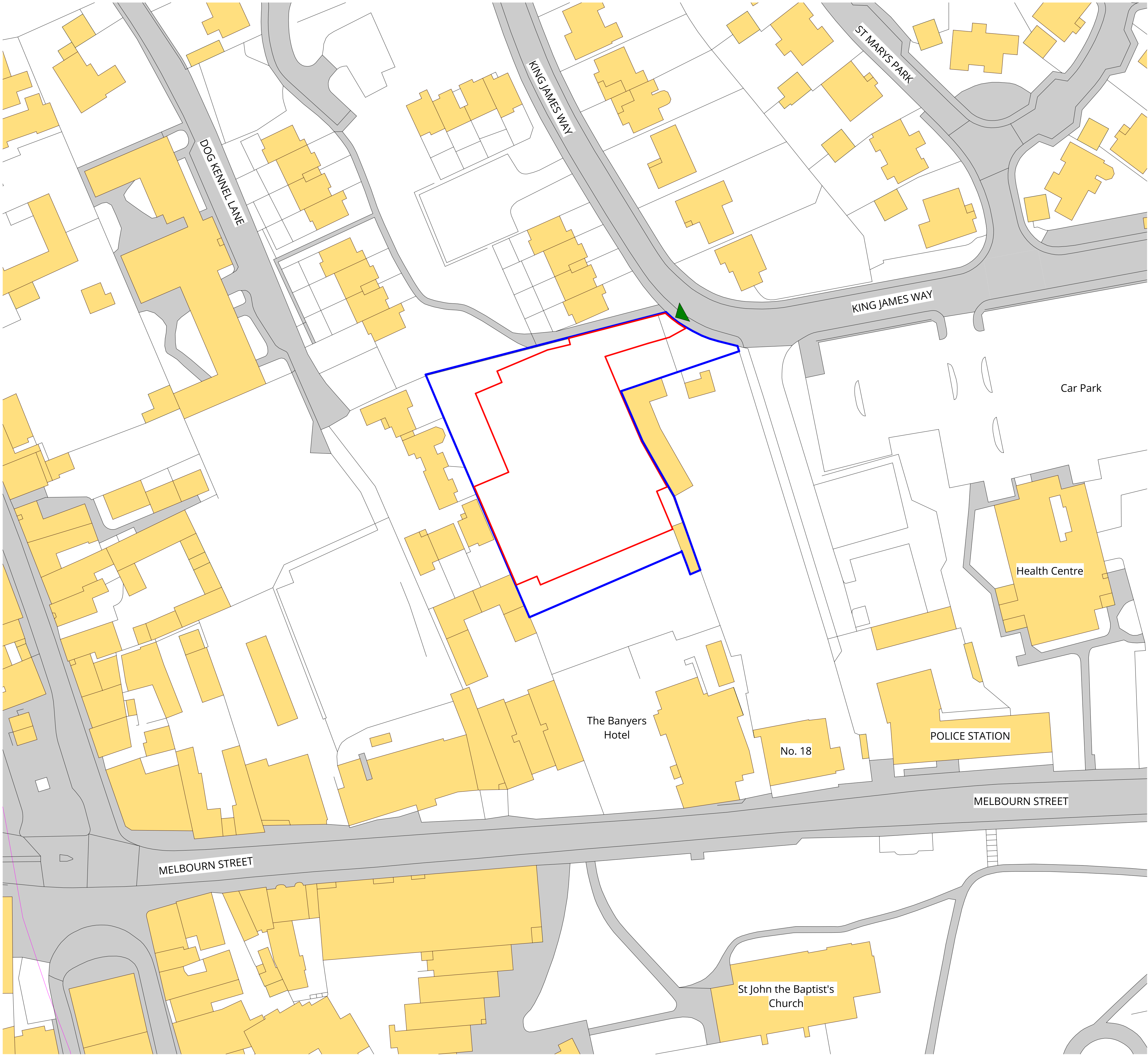
1 Site Location Plan Scale 1 : 500
