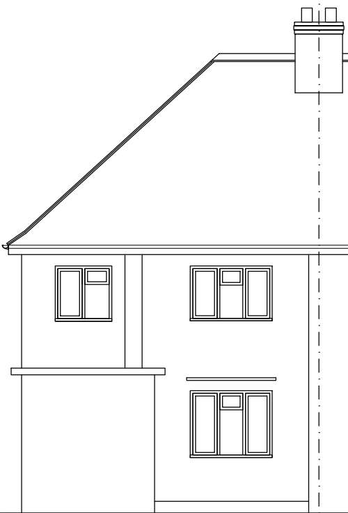
REAR ELEVATION
