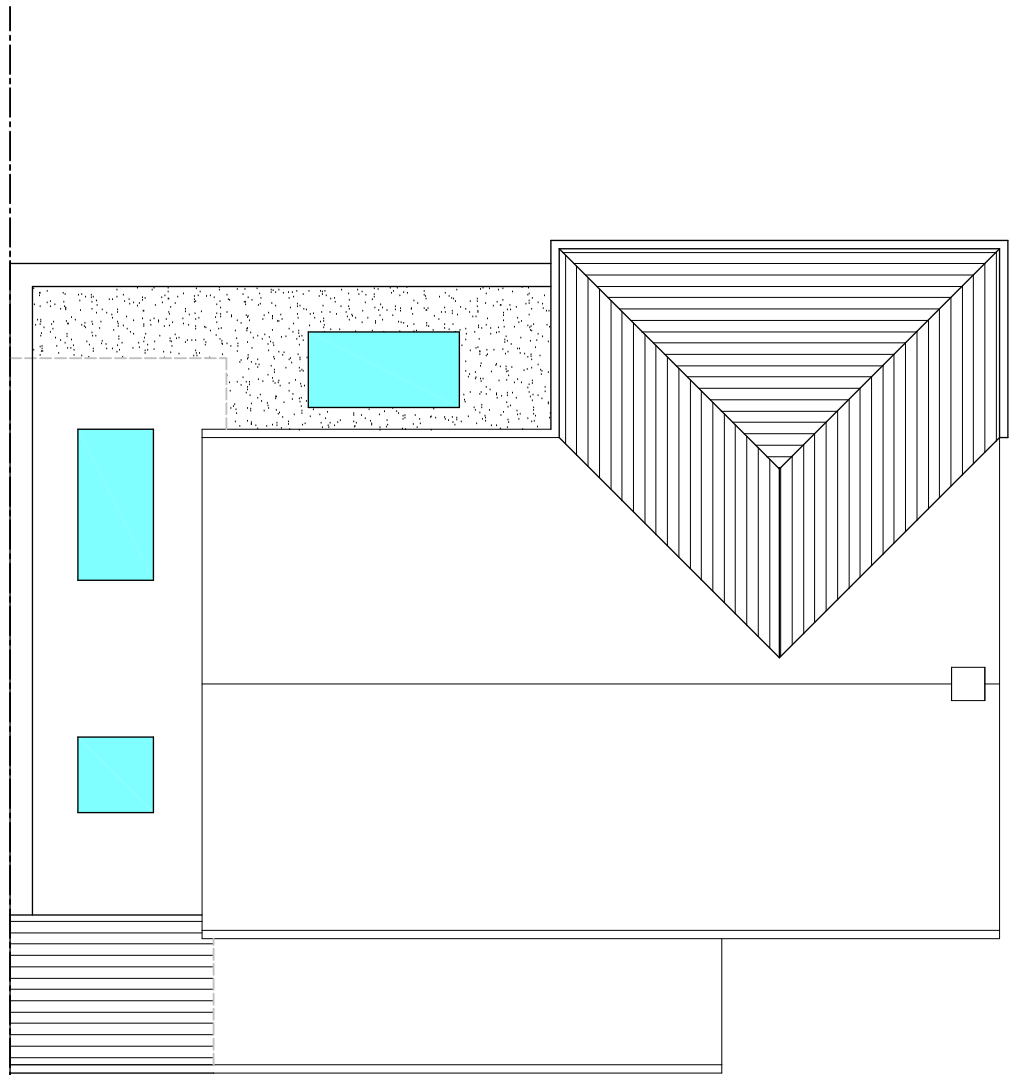
ROOF PLAN
