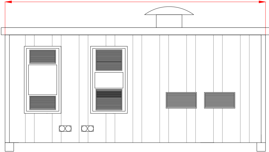
REAR View
