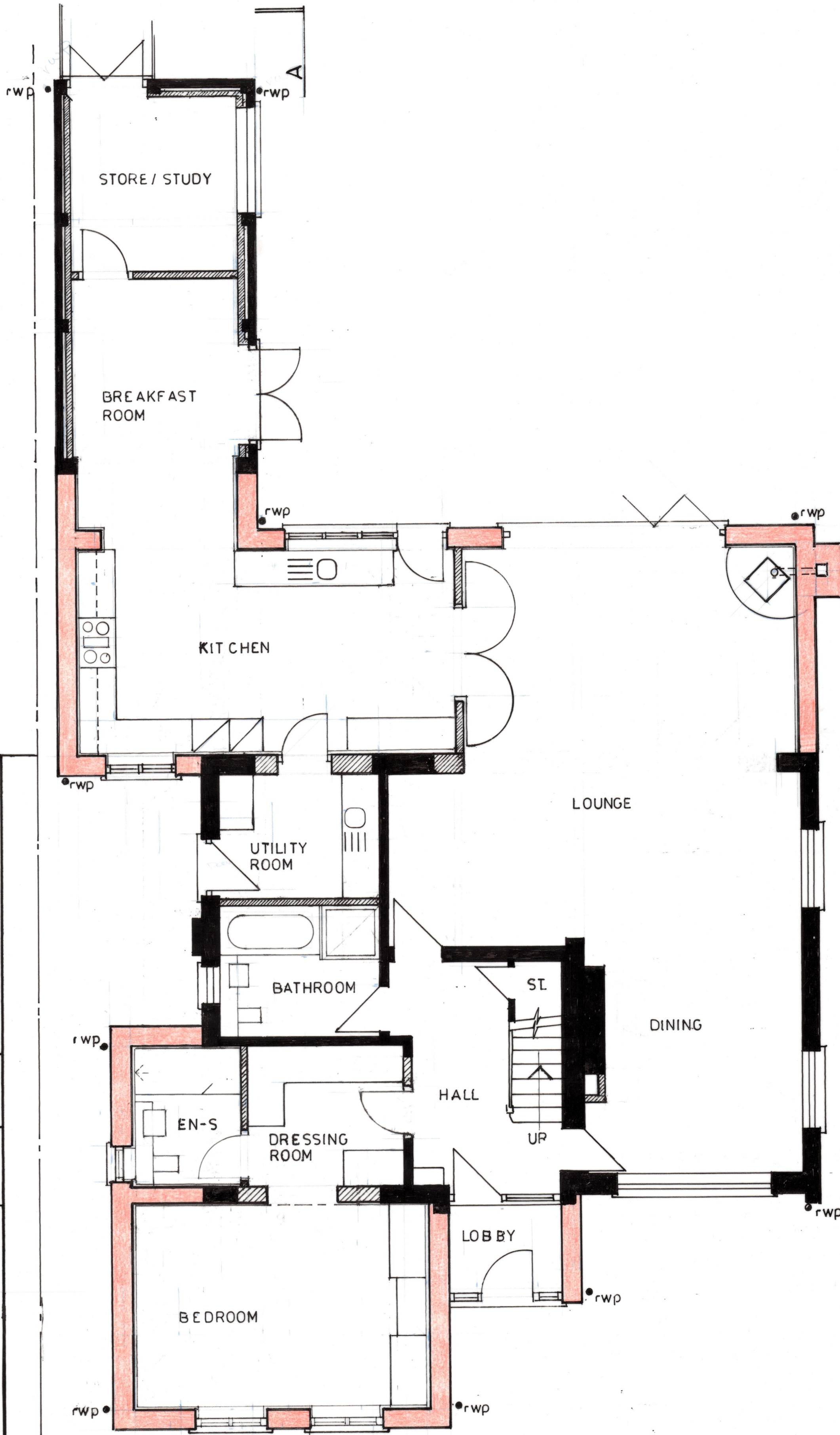
GROUND FLOOR LAYOUT
