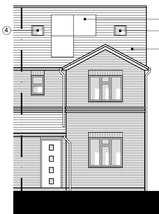
FRONT ELEVATION (A-A)
