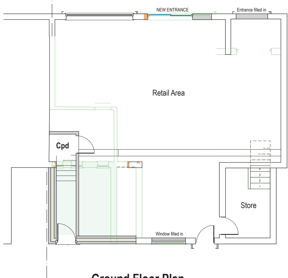
Ground Floor Plan (9m2)
