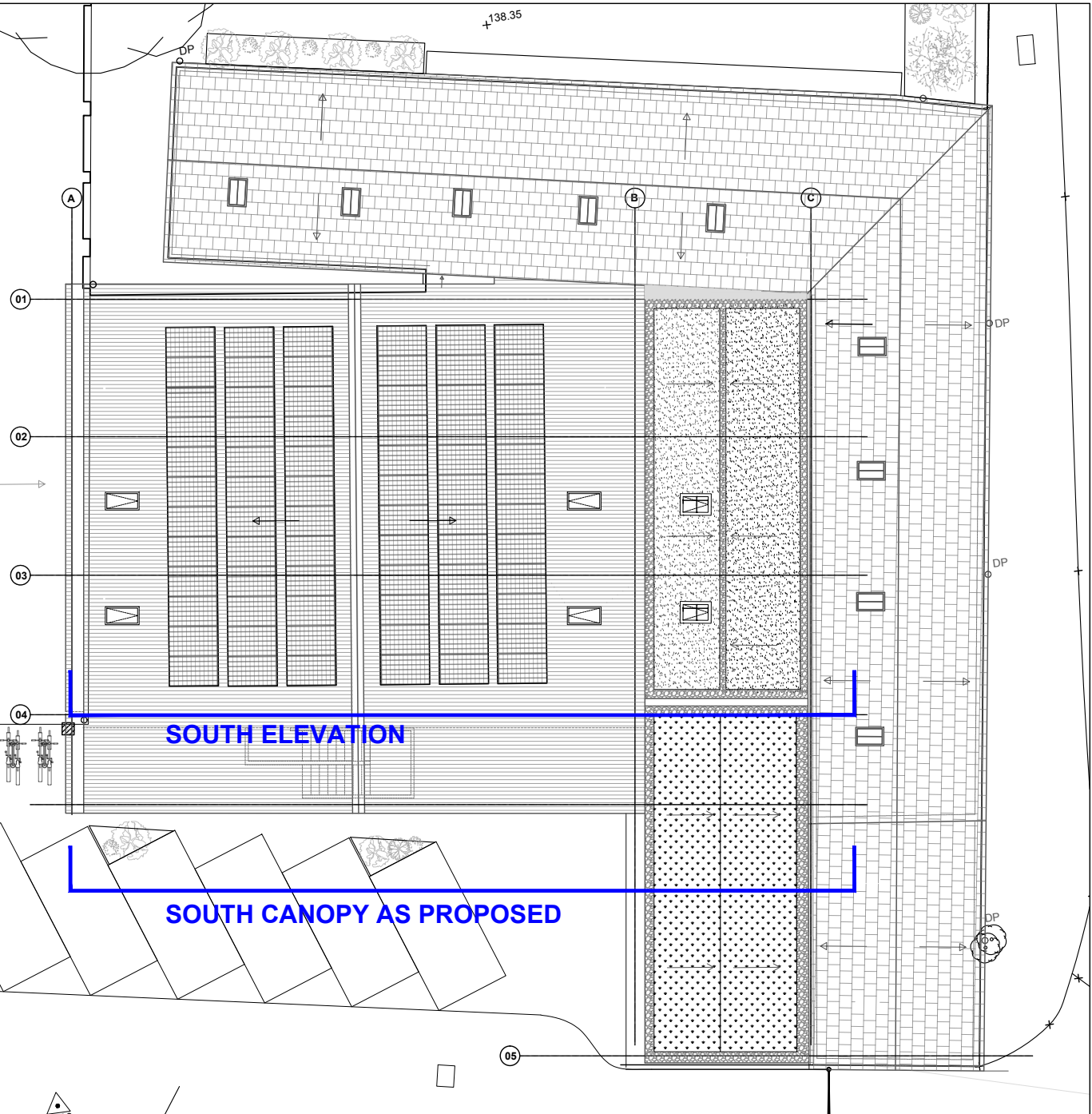
Key plan 1/200
