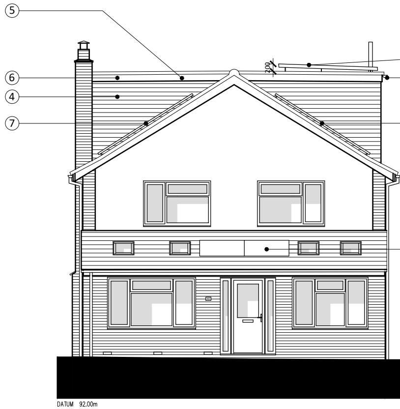
FRONT ELEVATION (A-A)
