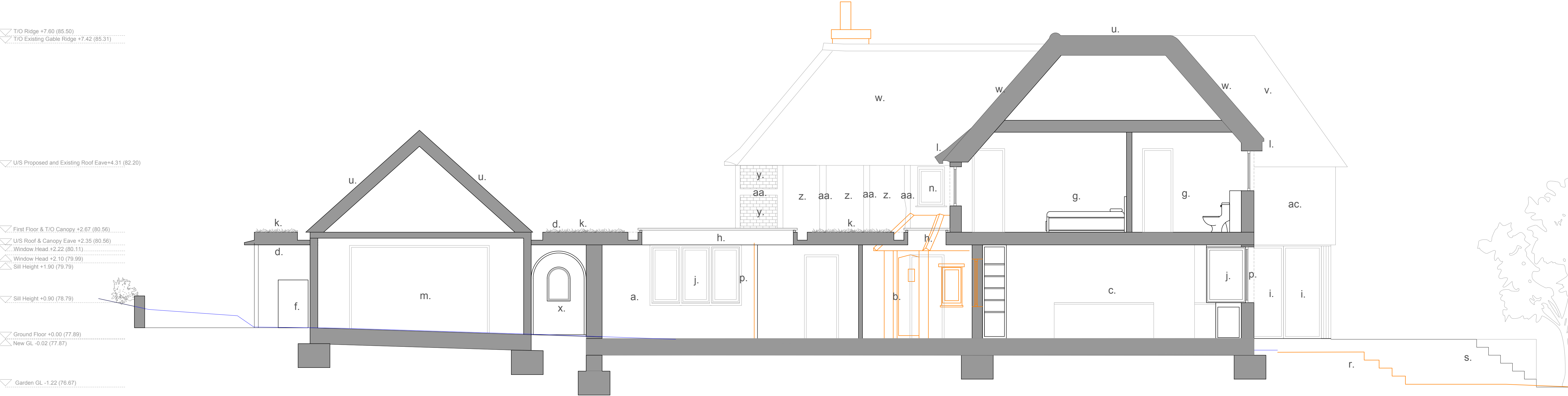
Section BB'
