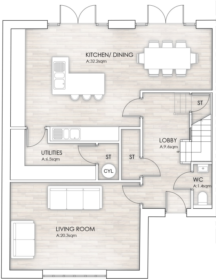
Proposed Ground Floor Plan 0 1 2 3 4 5m Scale GIA: 158.1sqm (1701sqft)
