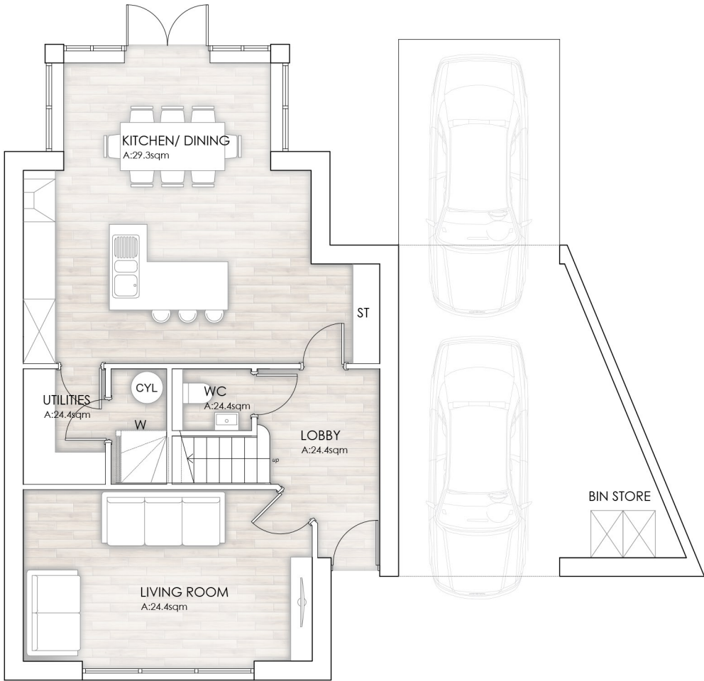
Proposed Ground Floor Plan 0 1 2 3 4 5m Scale GIA: 150sqm (1615sqft)
