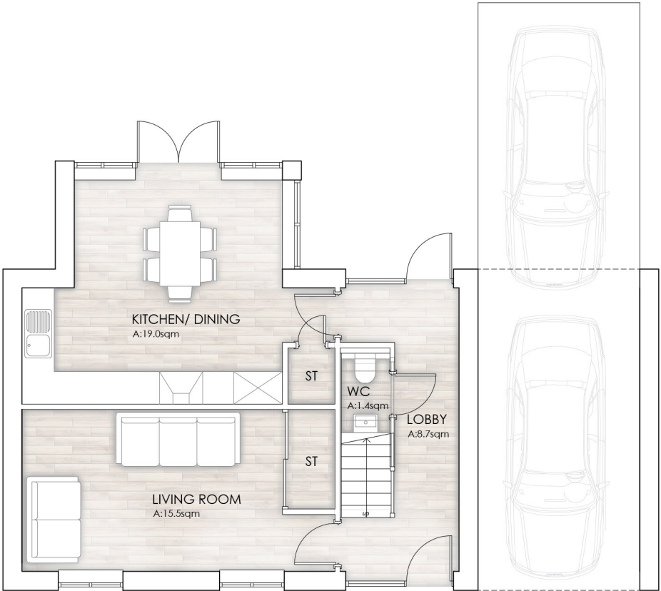
Proposed Ground Floor Plan 0 1 2 3 4 5m Scale GIA: 110.5sqm (1198sqft)
