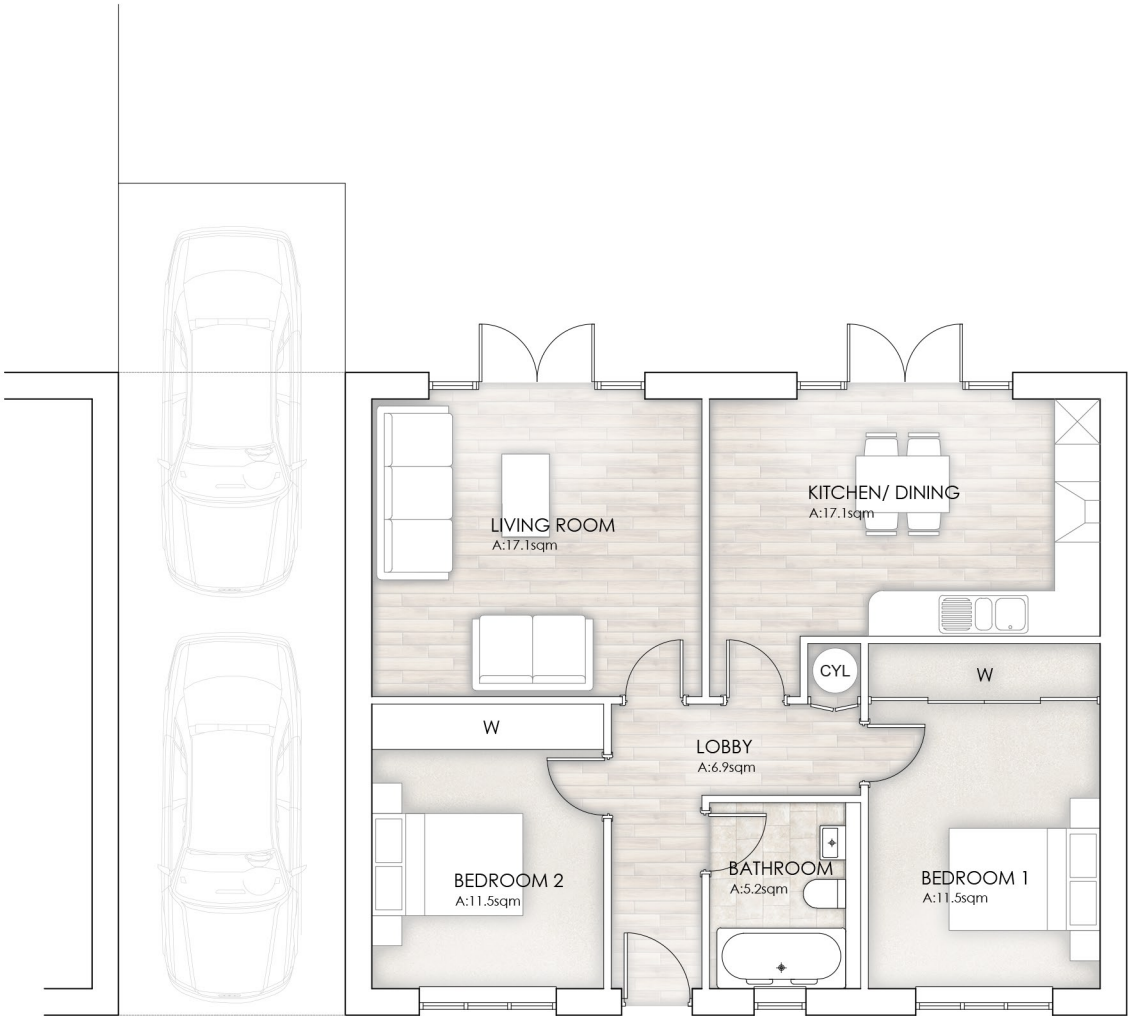
Proposed Ground Floor Plan 0 1 2 3 4 5m Scale GIA: 75.1sqm (808sqft)
