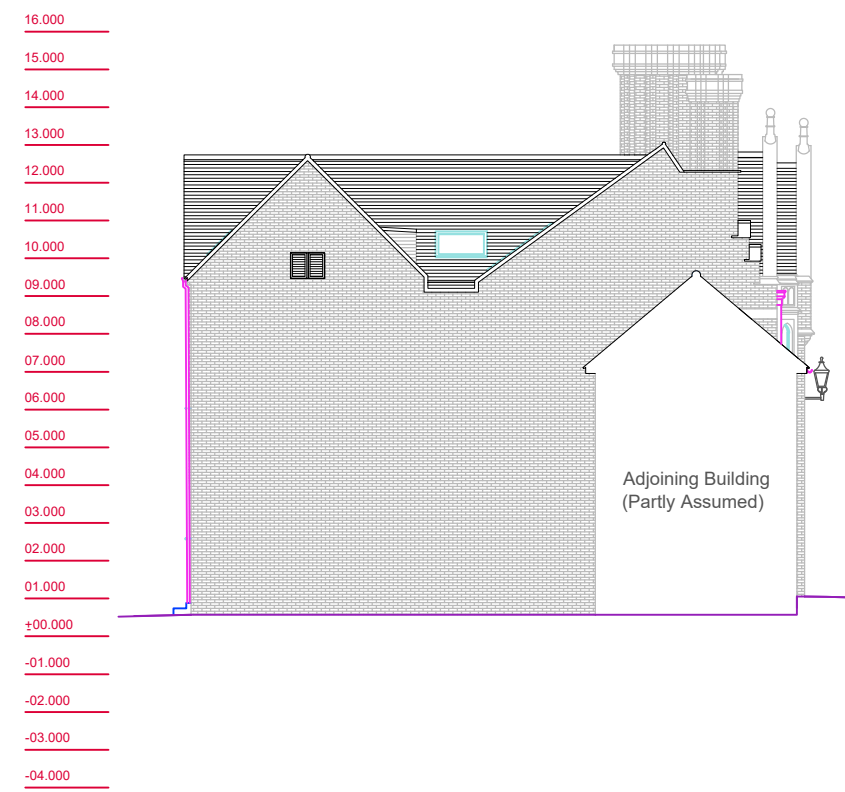
Left Elevation
