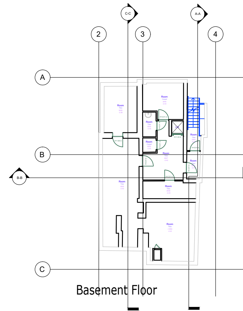
Basement Floor
