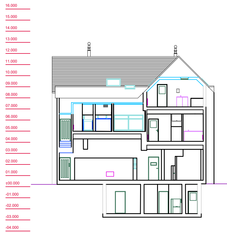
Section B-B
