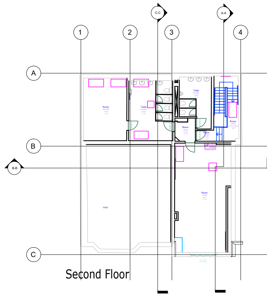
Second Floor
