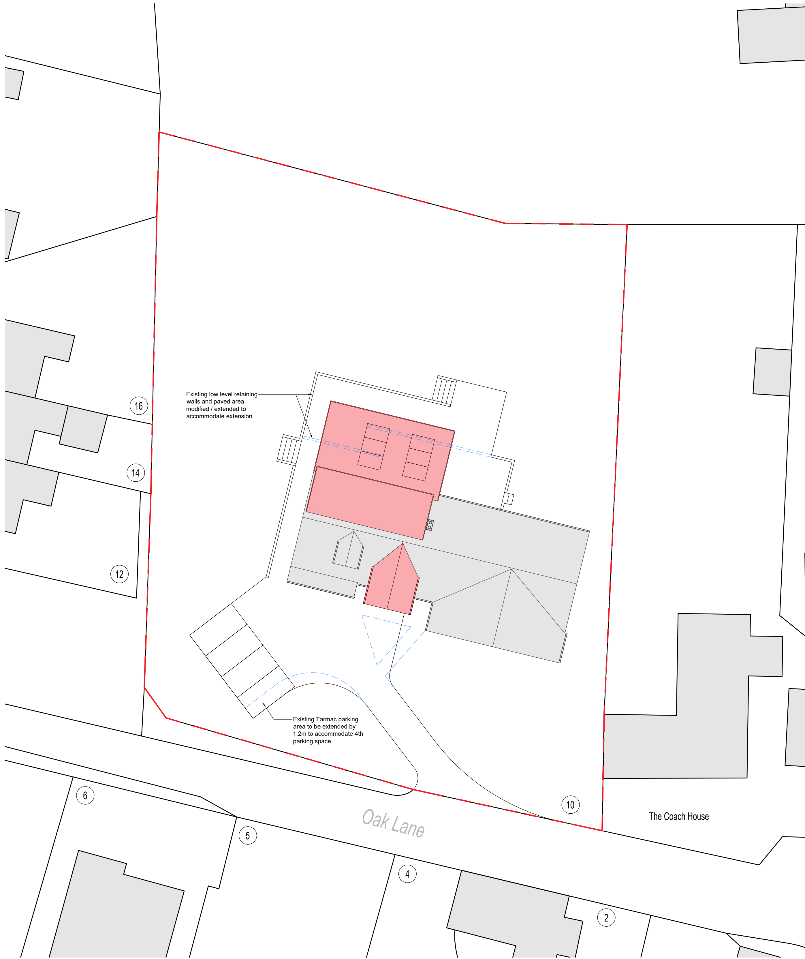
PROPOSED BLOCK PLAN @ 1 TO 200
