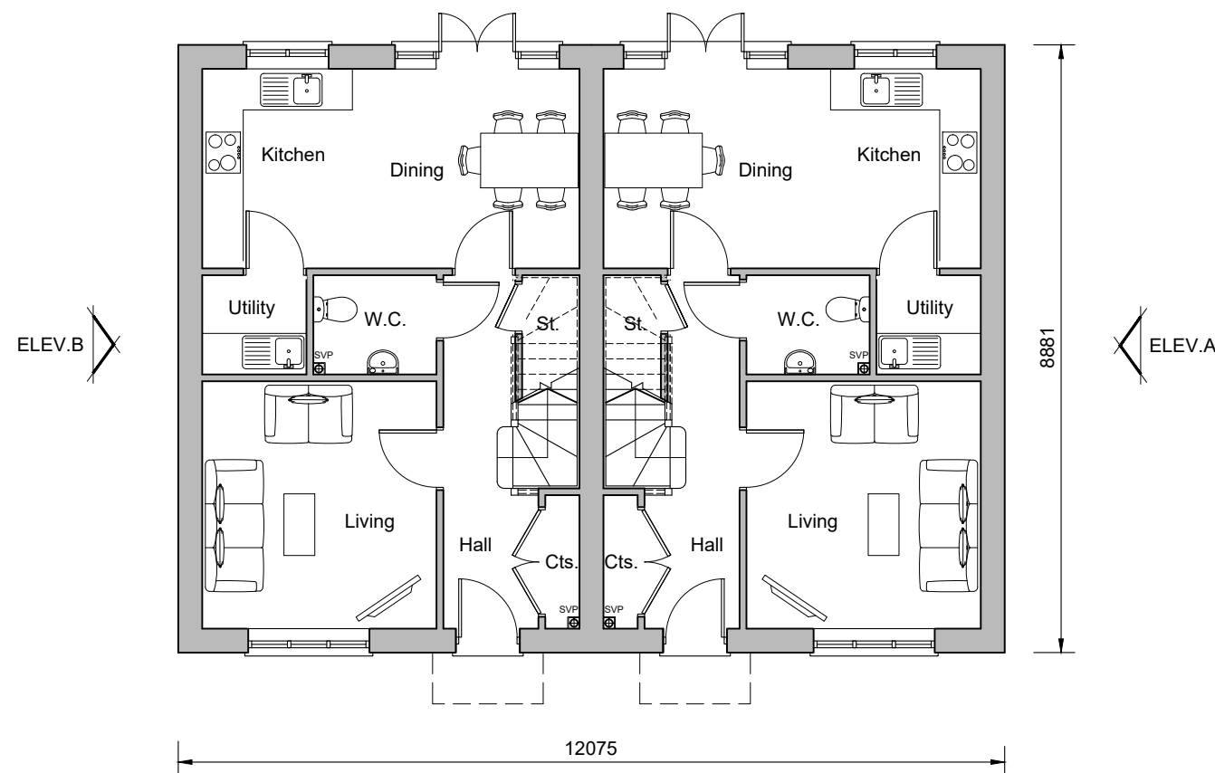
Ground Floor Plan Plots 62-63 Area - 83.9m2 (903sqft)
