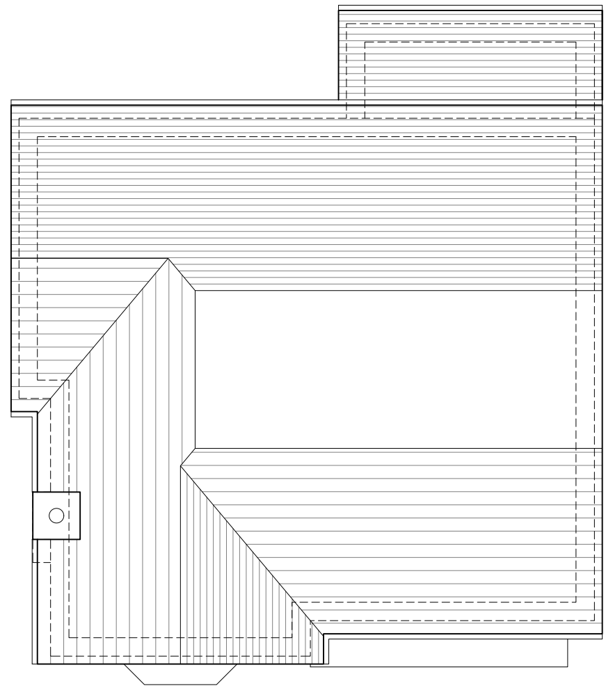
Roof Plan
