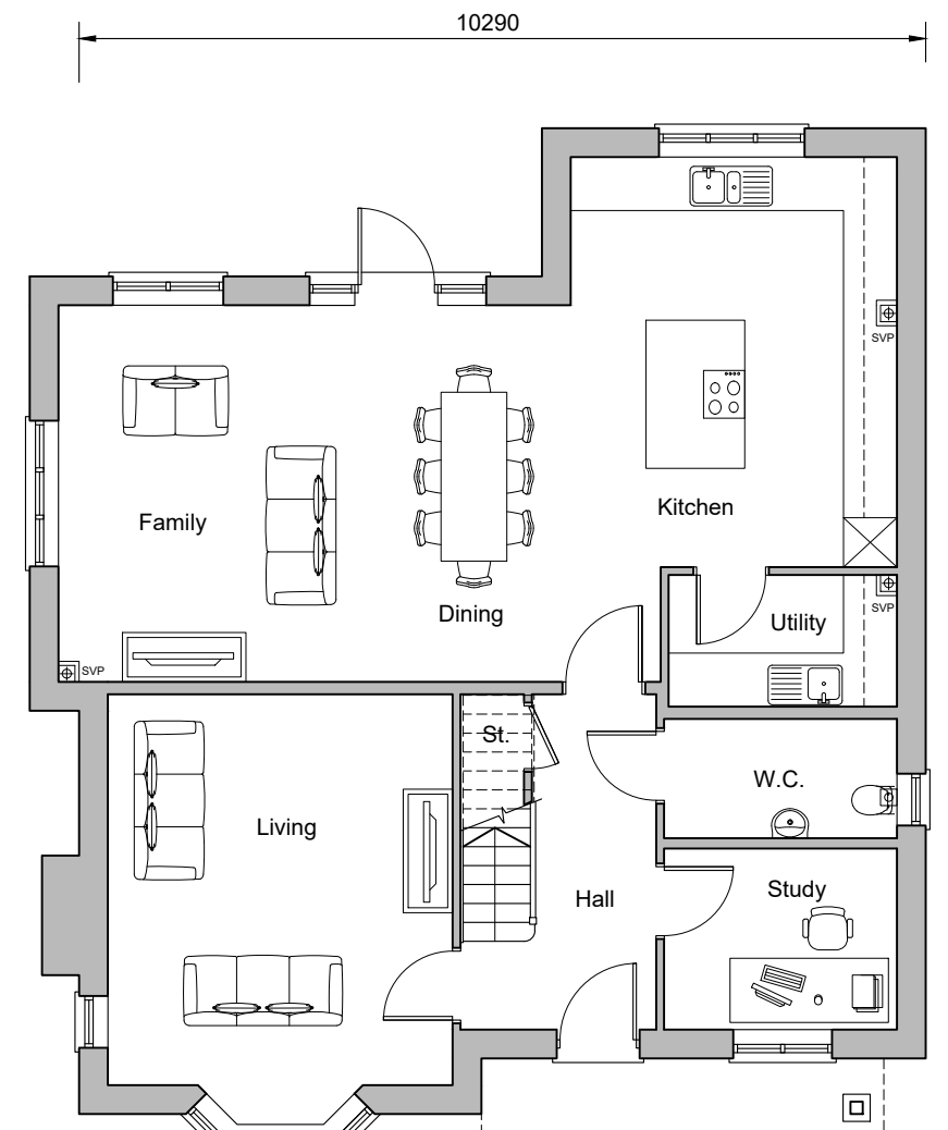
Ground Floor Plan Plots 64 and 82 Area - 187.8m 2 (2,021sqft)
