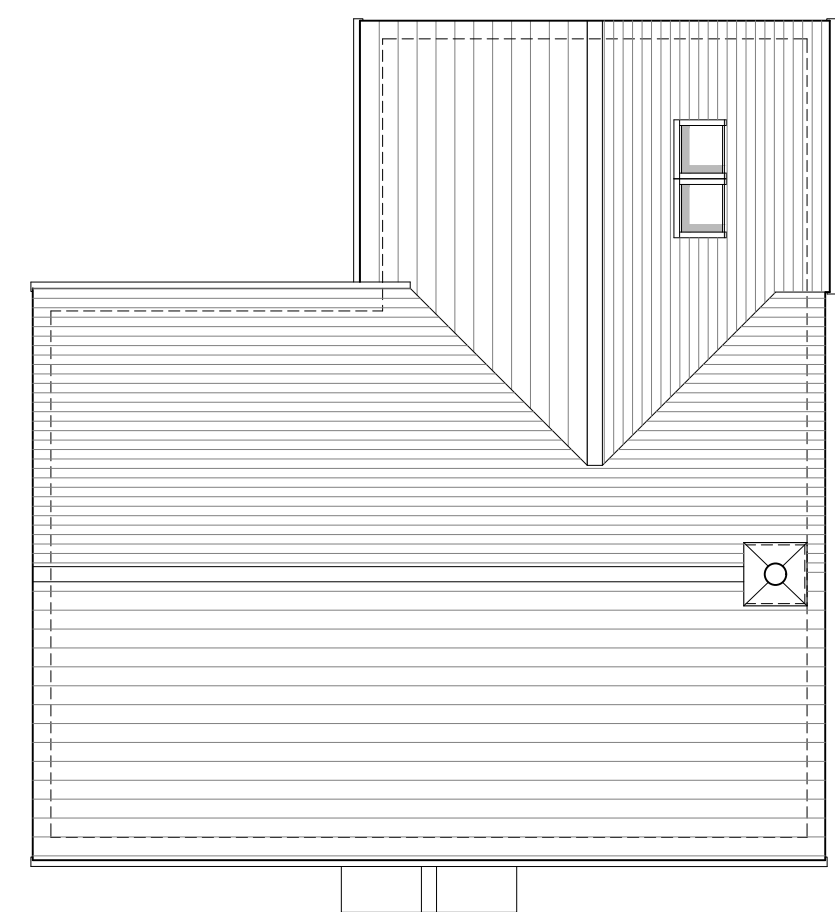
Roof Plan
