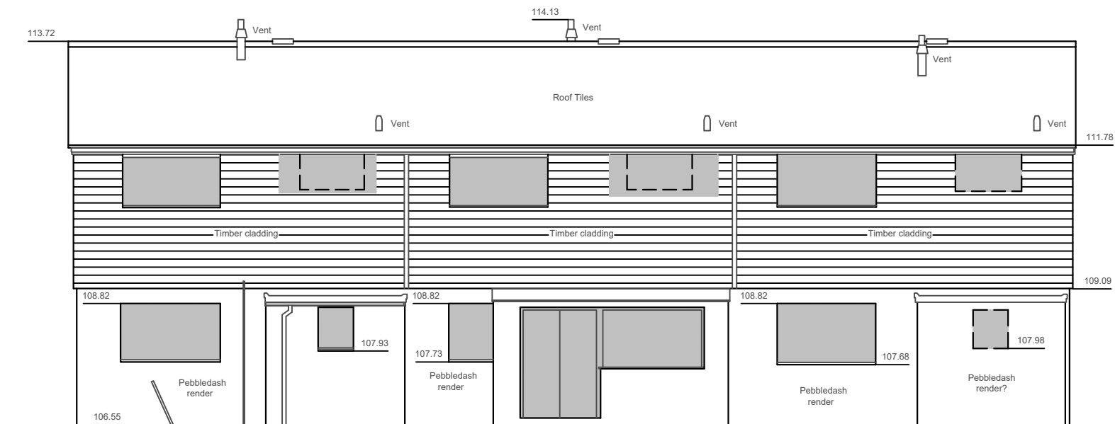
105.00m AOD Elevation C - Rear
