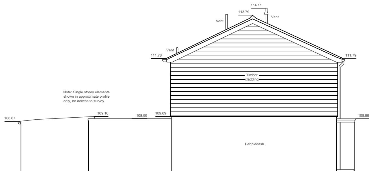
105.00m AOD Elevation D
