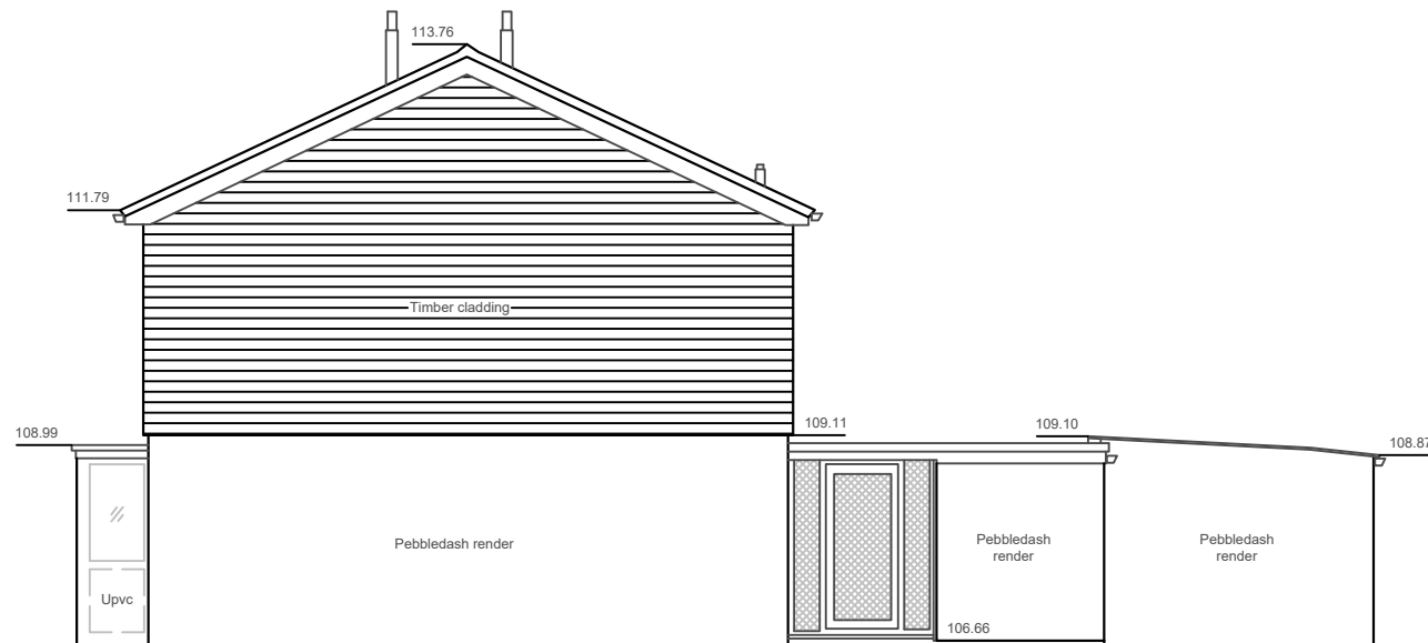
105.00m AOD Elevation B
