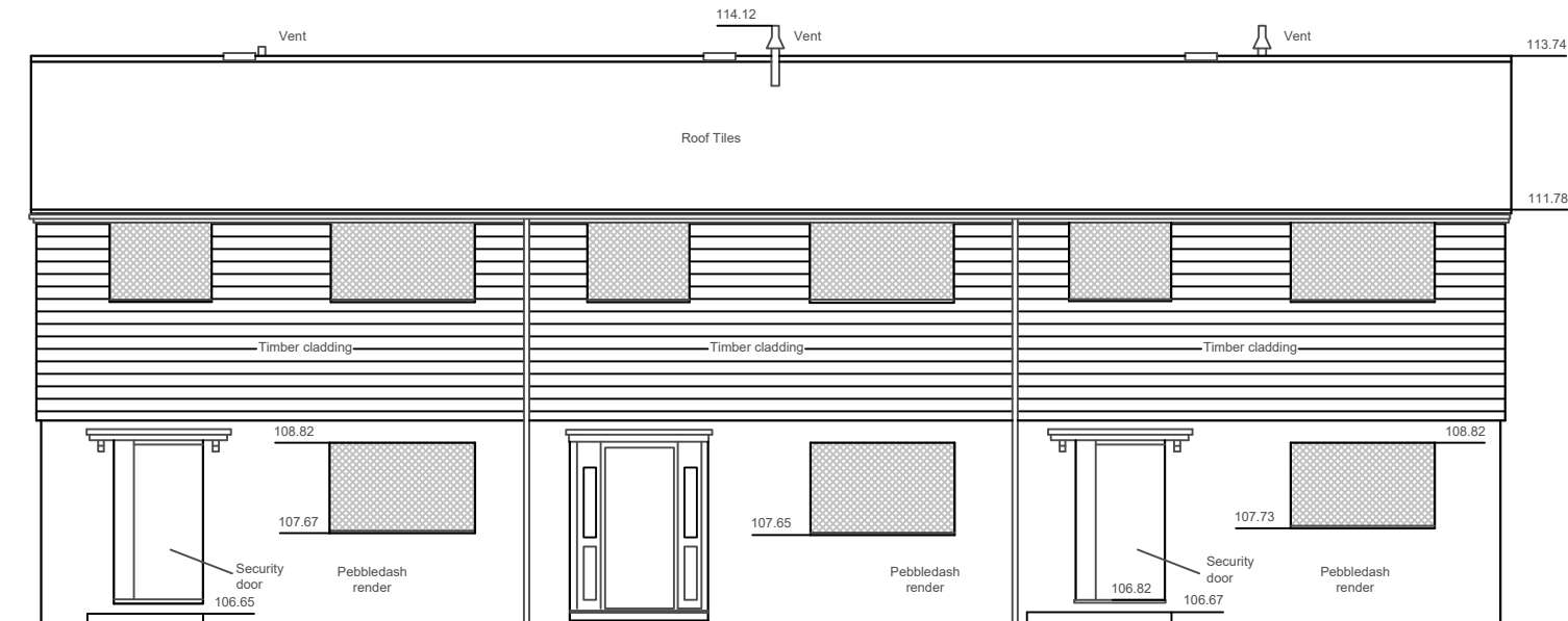
105.00m AOD Elevation A - Front
