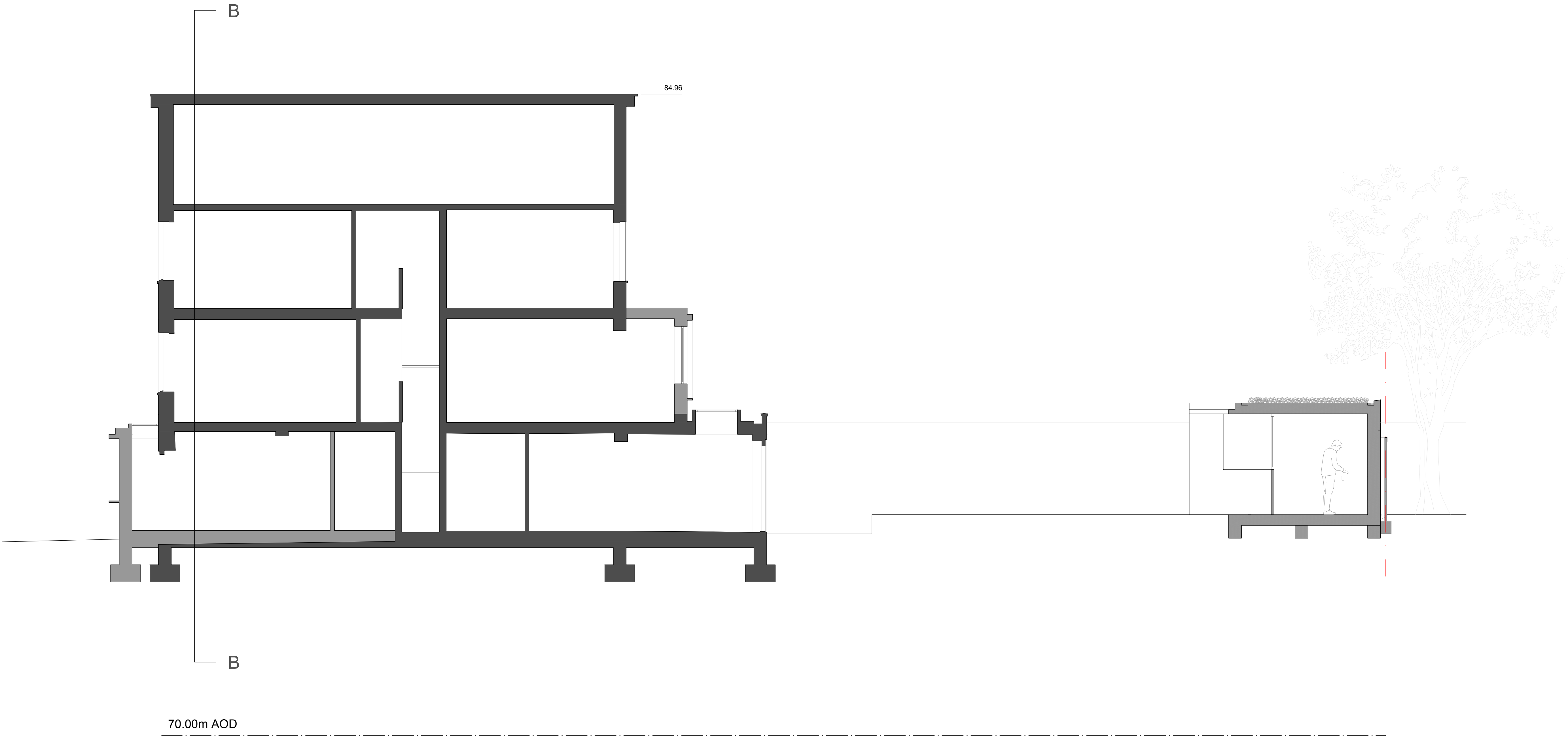
Proposed Section AA
