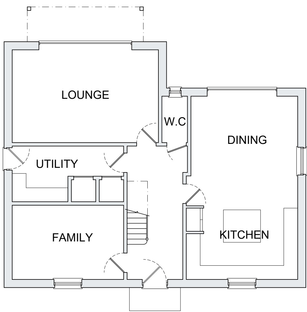
GROUND FLOOR 1:100 PLOT 5
