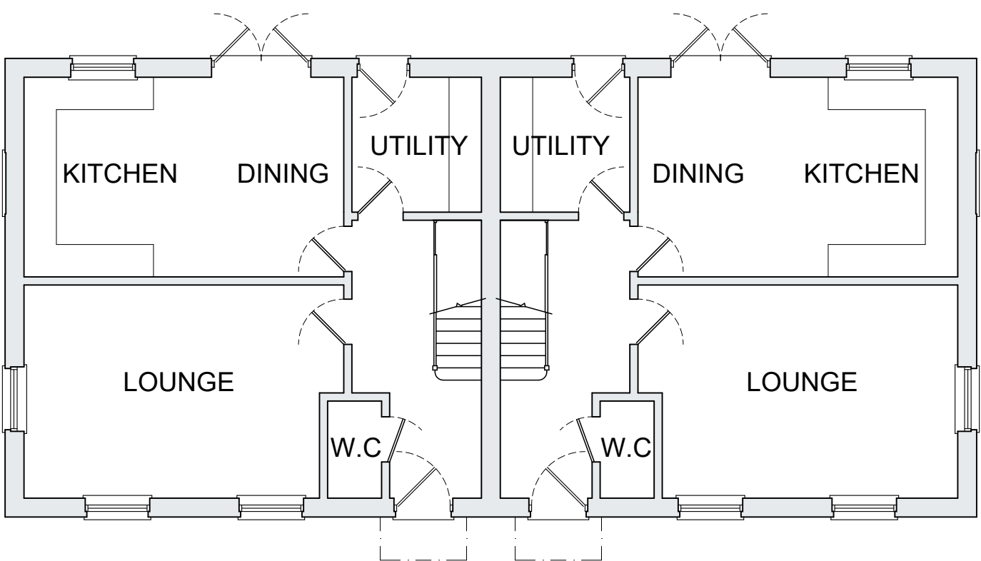
GROUND FLOOR 1:100 PLOTS 6 & 7
