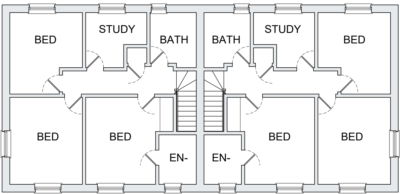
FIRST FLOOR 1:100
