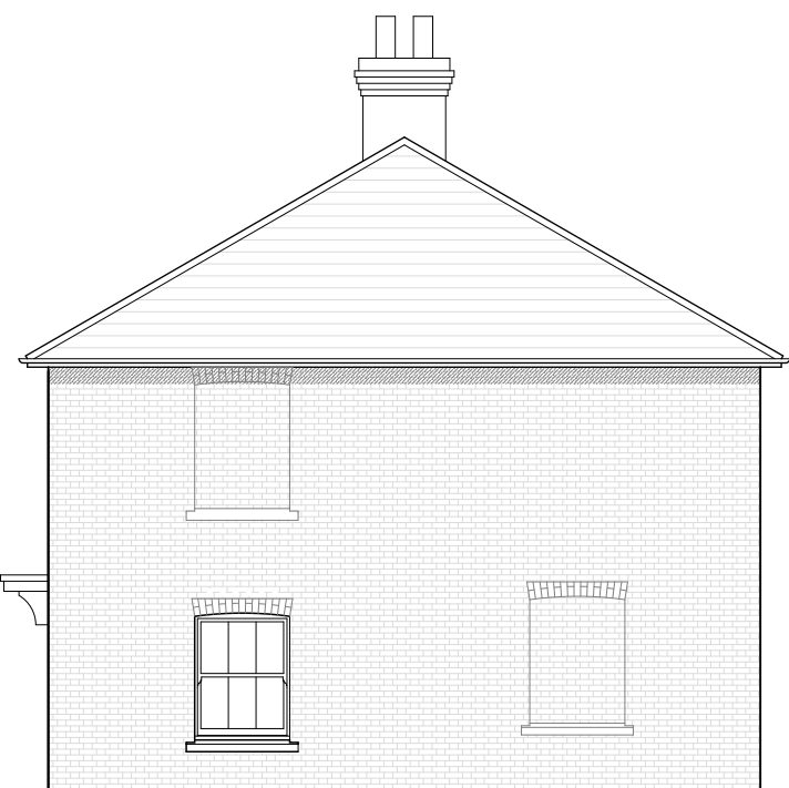
SOUTH ELEVATION 1:100
