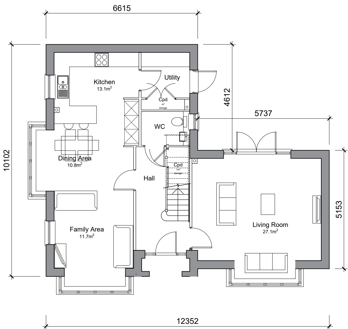
Ground Floor Plan 4-Bed 6-Person House GIA: 164.5 sqm / 1771 sqft Storage: 5.3 sqm (3.0 sqm required)
