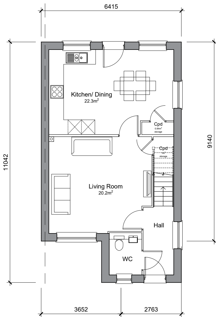
Ground Floor Plan 4-Bed 6-Person House GIA: 107.6 sqm / 1158 sqft Storage: 3.0 sqm (3.0 sqm required)
