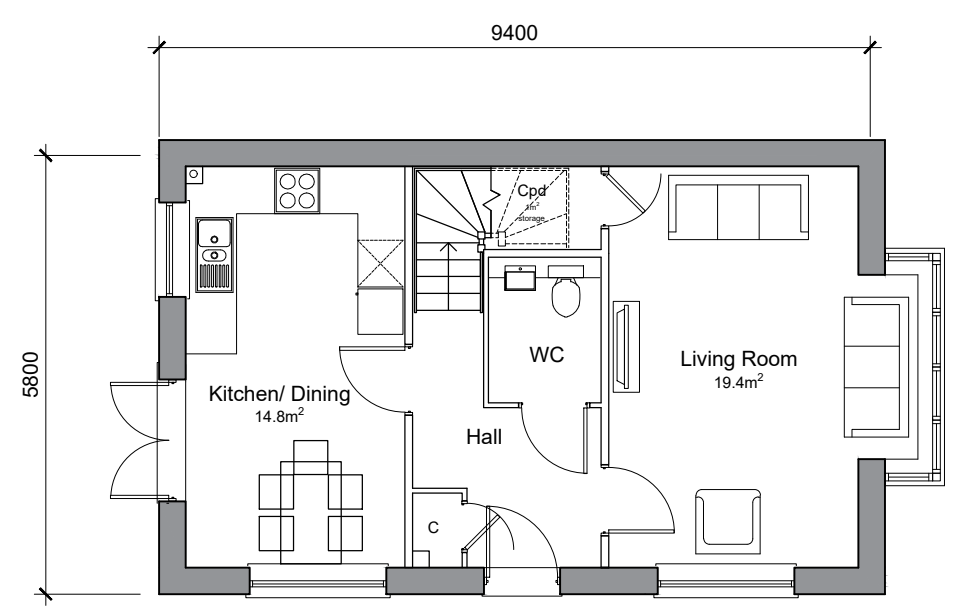
Ground Floor Plan 2-Bed 3-Person House GIA: 96.3 sqm / 1037 sqft Storage: 2.9 sqm (2.5 sqm required) Plots: 34 39 (handed)
