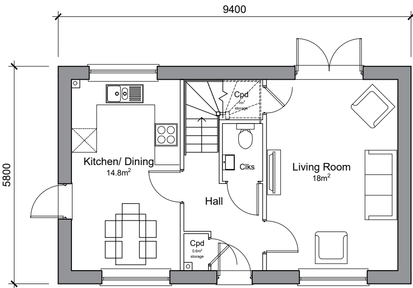
Ground Floor Plan 2-Bed 3-Person House GIA: 88.8 sqm / 956 sqft Storage: 2.9sqm (2.5 sqm required) Plots: 14 75 (handed)
