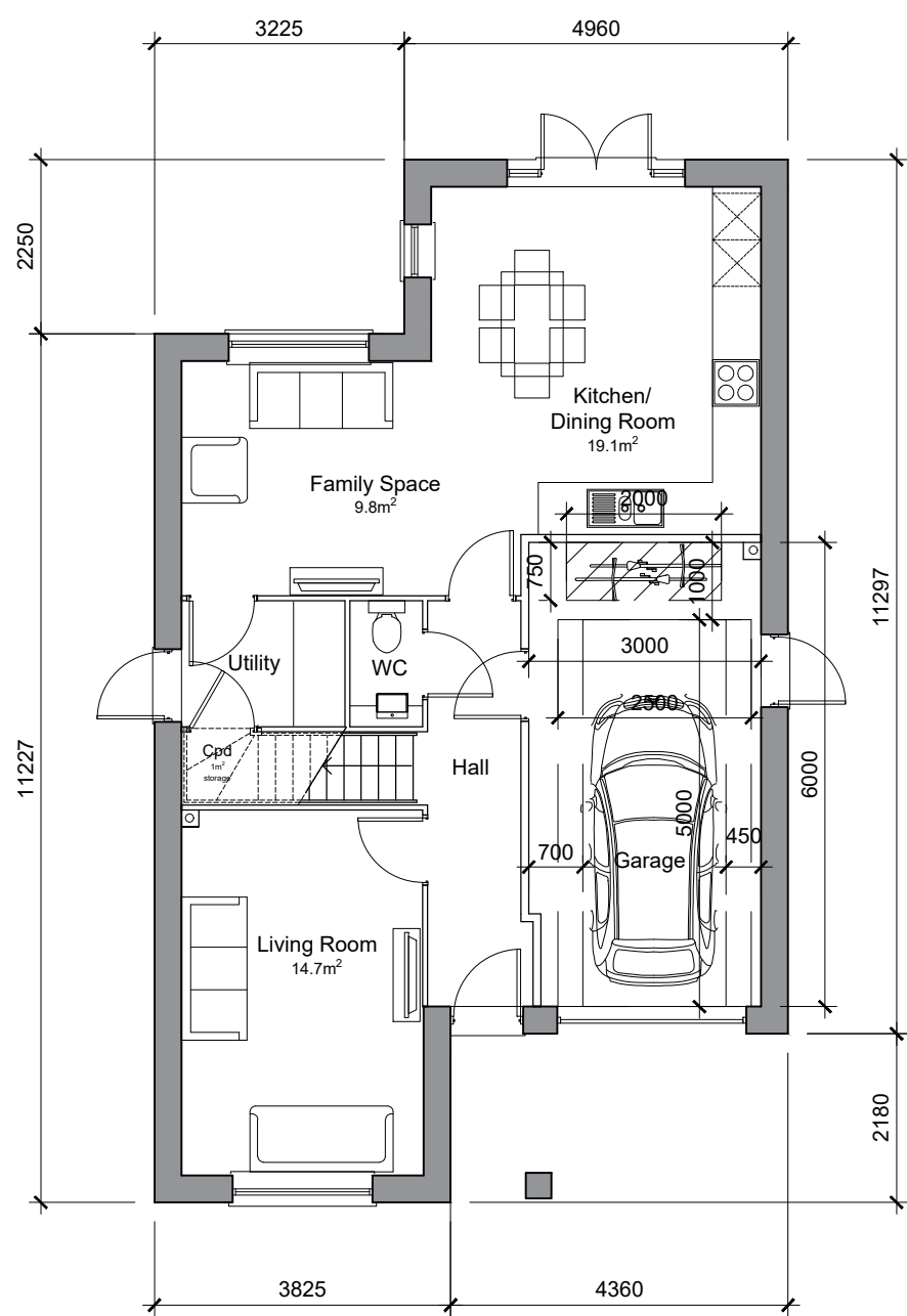
Ground Floor Plan 4-Bed 7-Person House GIA: 132.1 sqm / 1422 sqft Storage: 3.2 sqm (3.0 sqm required) Plots: 5, 6, 7, 20, 77 12, 27 (handed)
