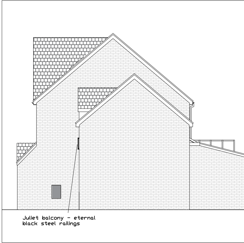
Proposed Side Elevations (1:100)
