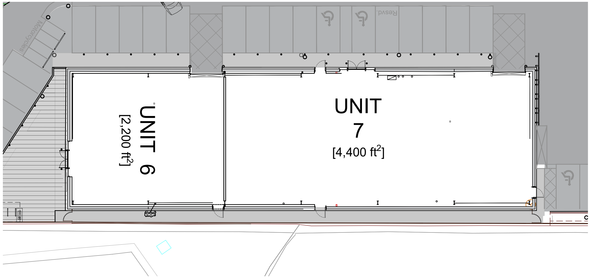
Units 6 & 7 Ground Floor Plan
