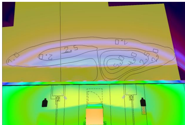
Figure 3.3.4 – Image showing the horizontal illuminance levels on the neighbouring gardens (calculation surface 1)
