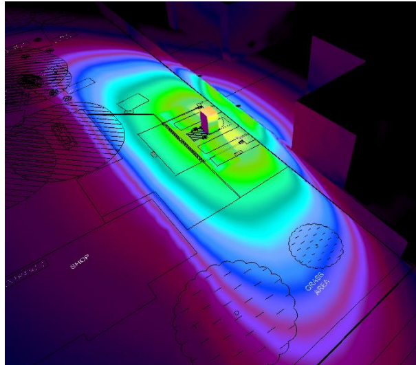
Figure 3.3.3 – Isoline plot (false colour rendering) layout for the preselected external column lighting scheme, with existing fence line
