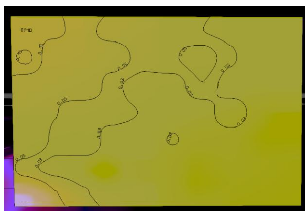
Figure 3.3.10 – Image showing the vertical illuminance levels on the facade of the nearest neighbouring proposed dwelling (calculation surface 3)
