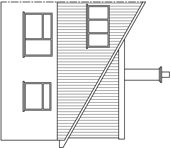
PROPOSED FRONT ELEVATION materials to match existing
