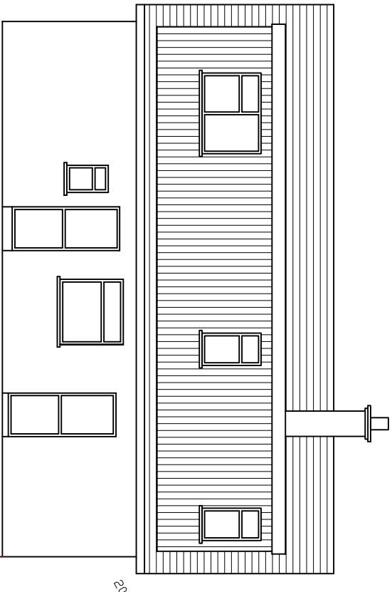
PROPOSED SIDE ELEVATION materials to match existing
