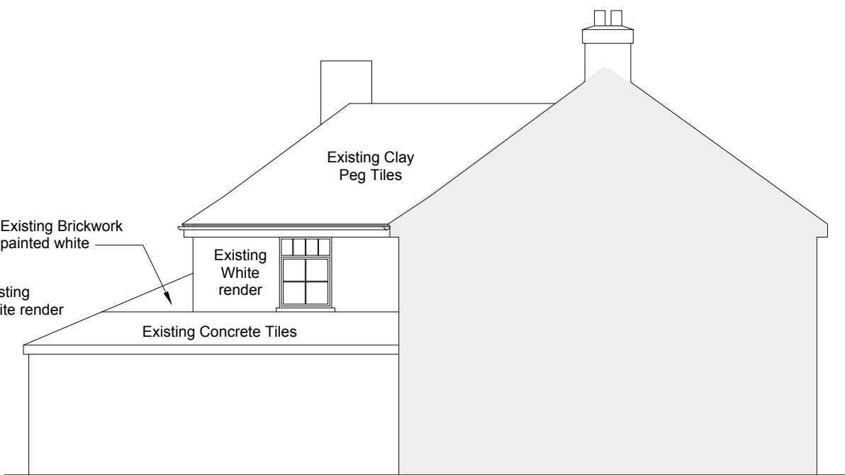
PRE-EXISTING SIDE (WEST) ELEVATION 1:100
