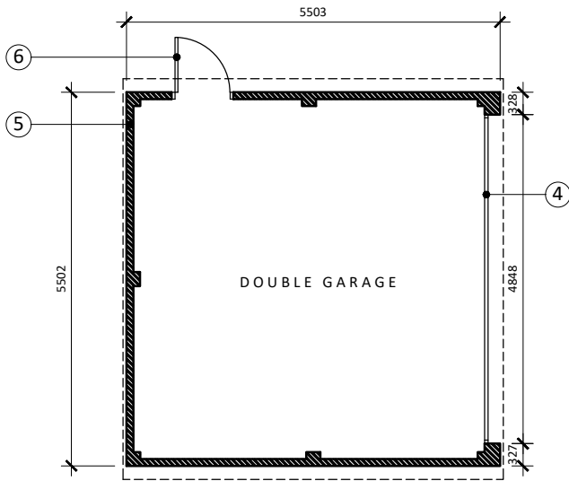
PROPOSED GARAGE PLAN
