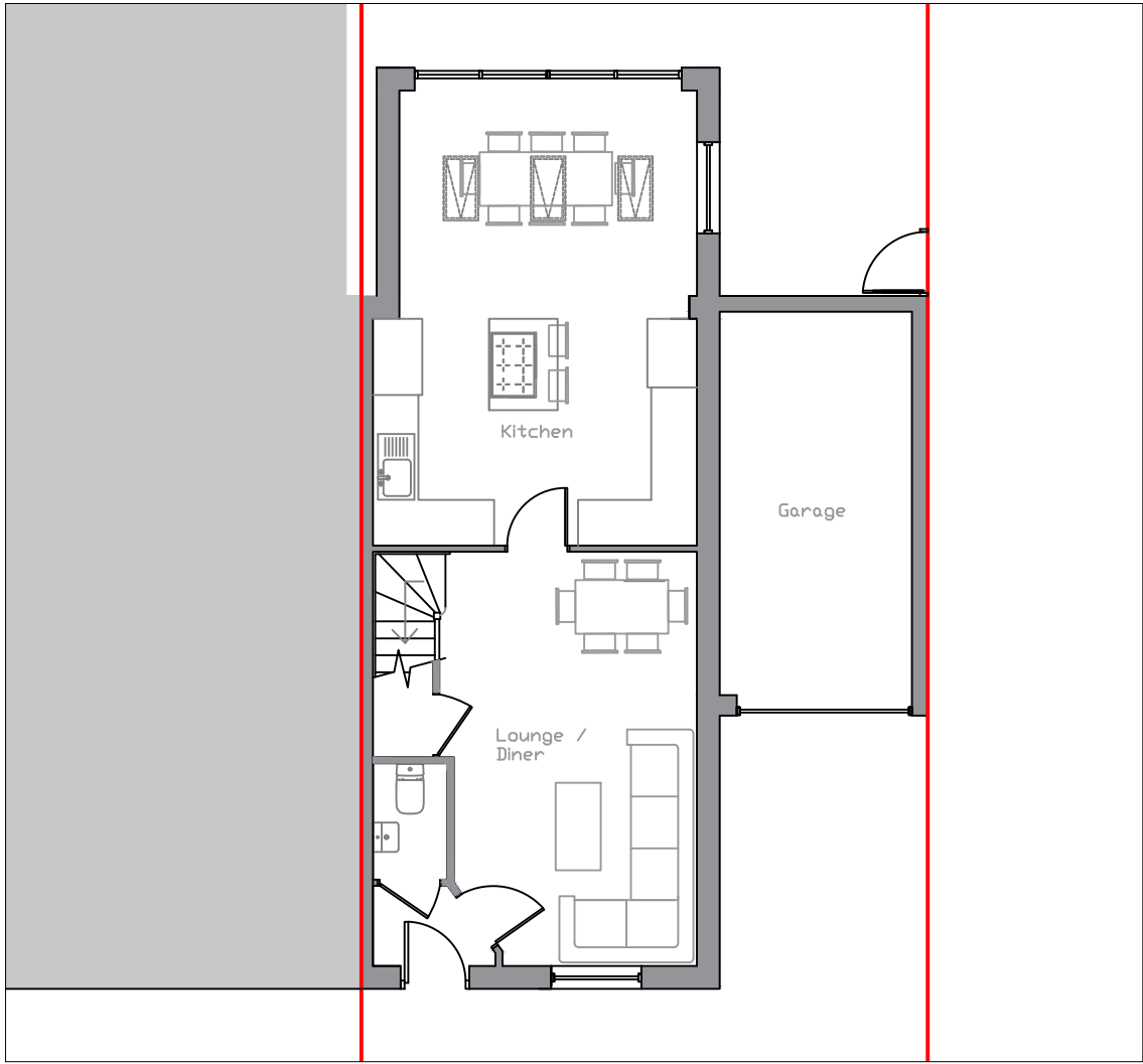
Ground Proposed
