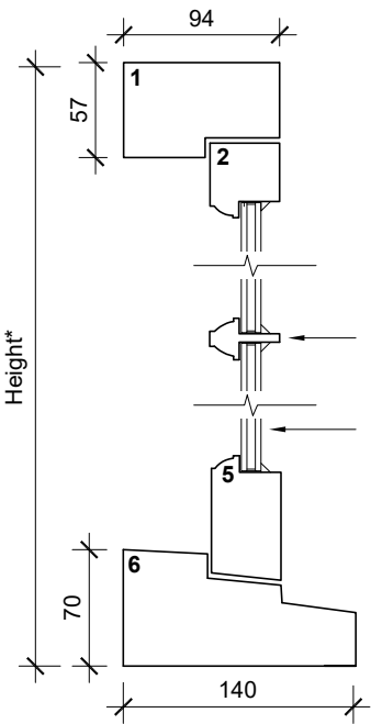
Typical Window - detail section 1:5
