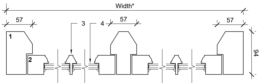
Typical Window - Detail Plan 1:5
