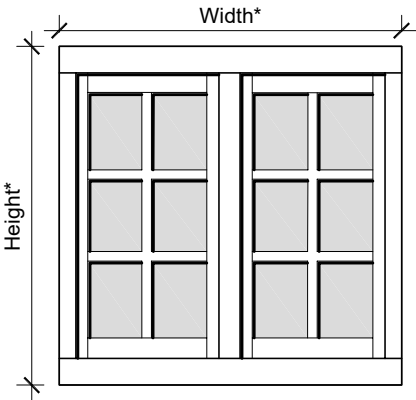
Typical Window Elevation 1:20
