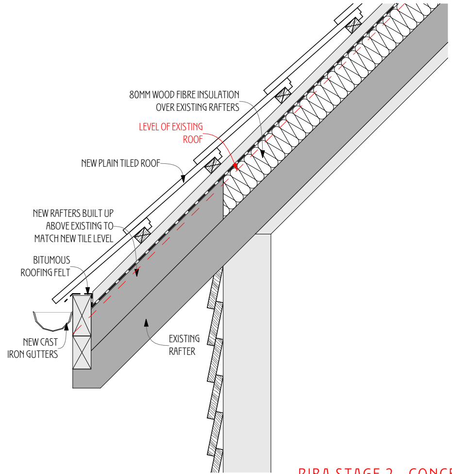
S-02 Roof Detail 2 Section 1:10
