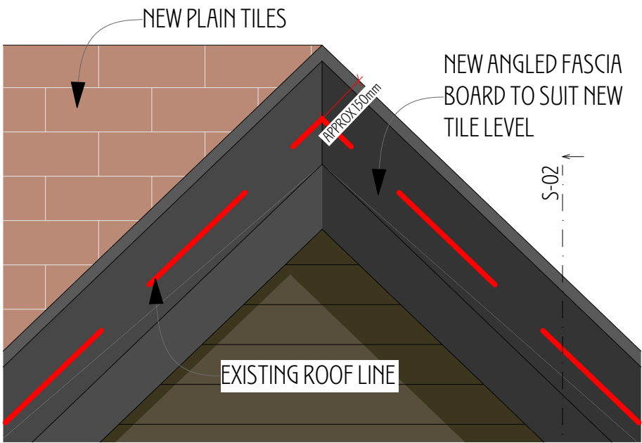
2 Proposed Roof Detail 1 1:10
