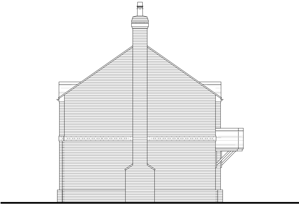
SIDE ELEVATION (1:100)
