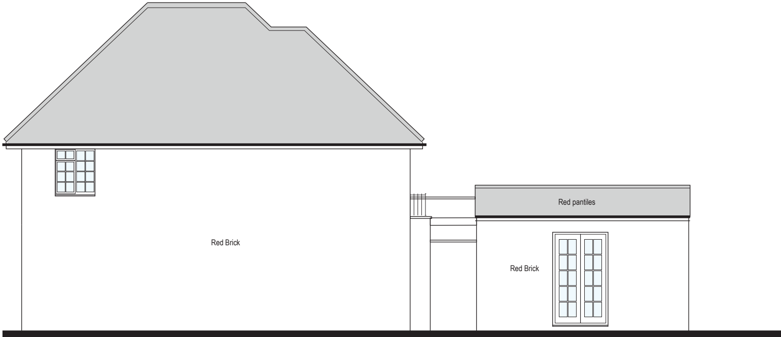
Side Elevation
