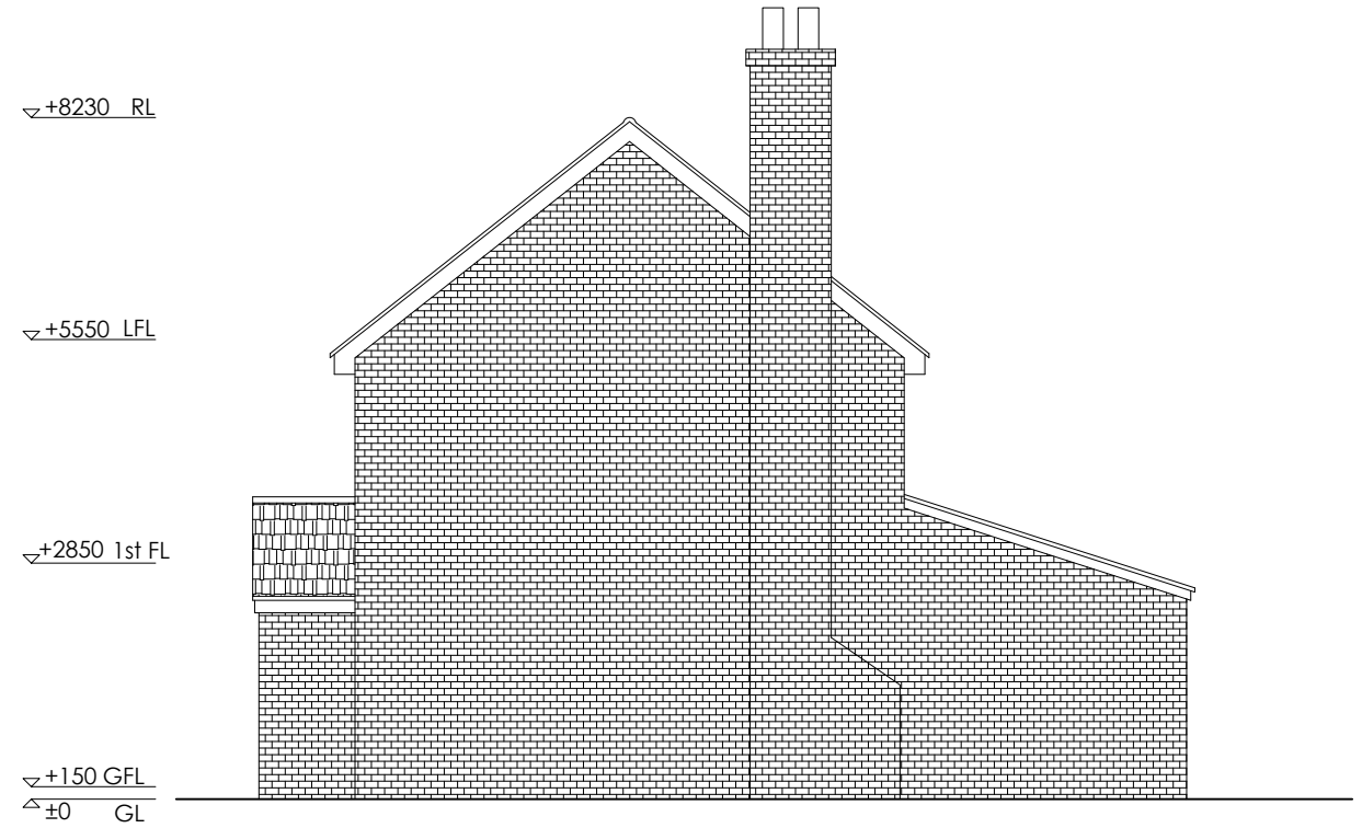
02 A-305 EXISTING RIGHT ELEVATION SCALE- 1:100@A3
