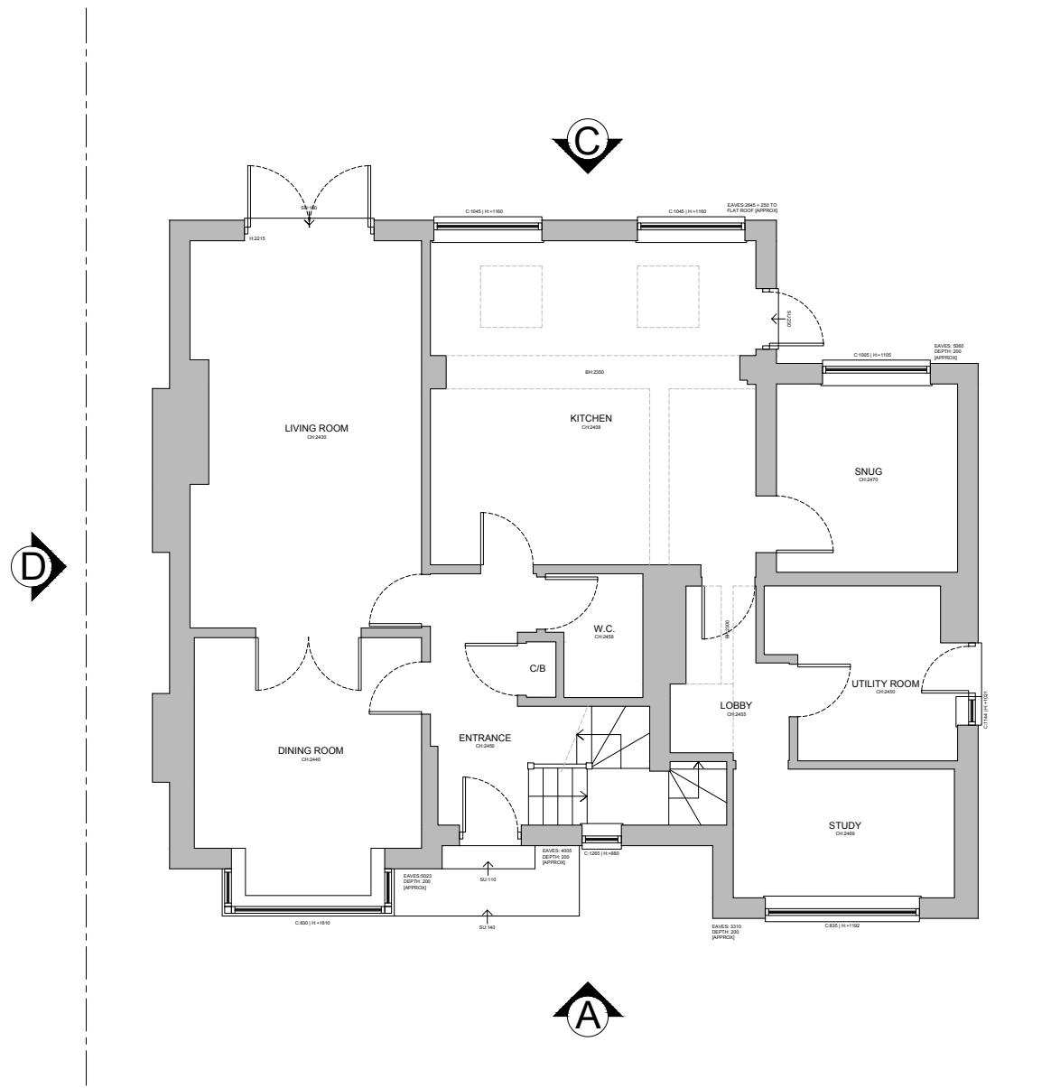
Pre-existing Ground Floor Plan
