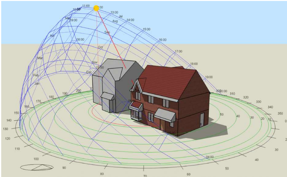
Image 4: North East Perspective
