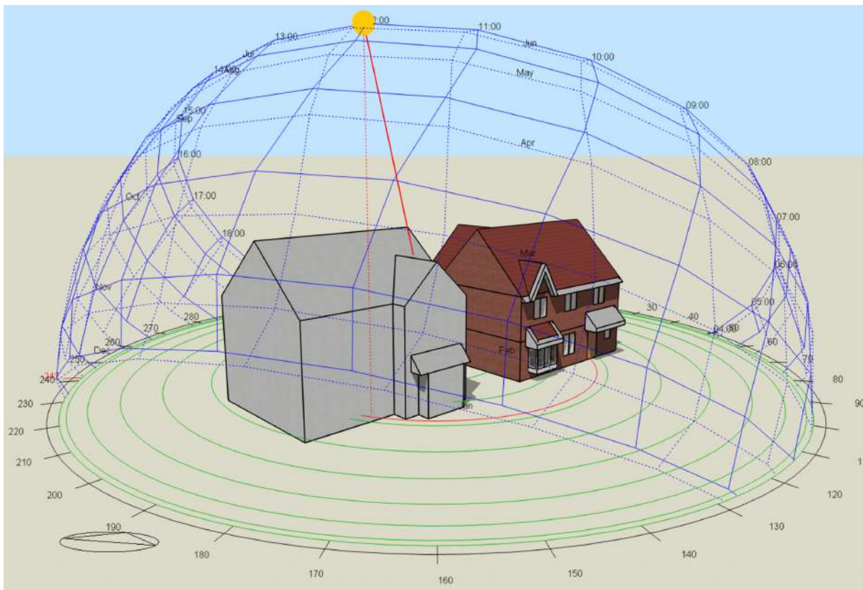
Image 5: South East Perspective
