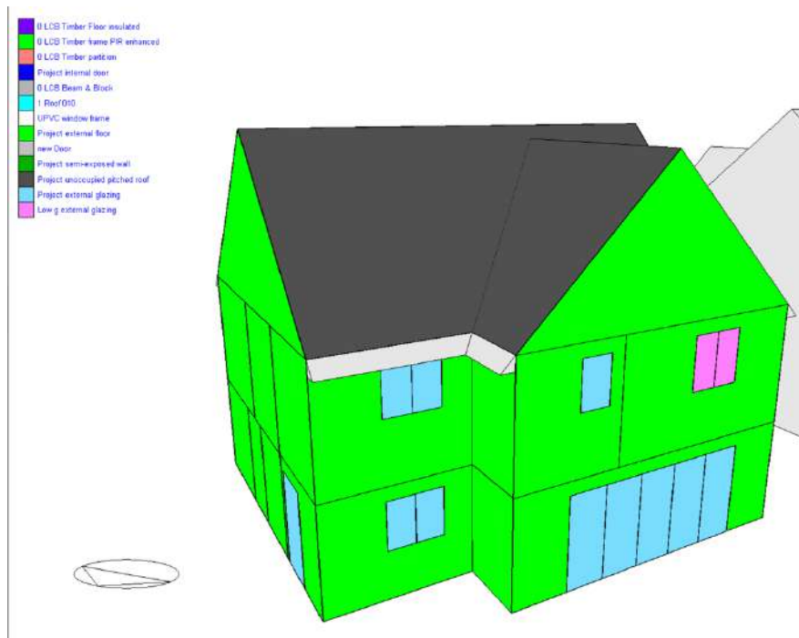
Figure 2: Rear elevation showing solar glazing to bedroom windows
