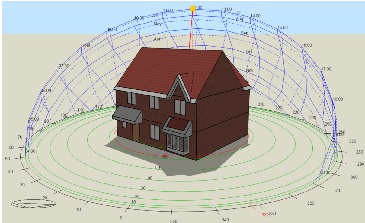
Image 4: North Perspective
