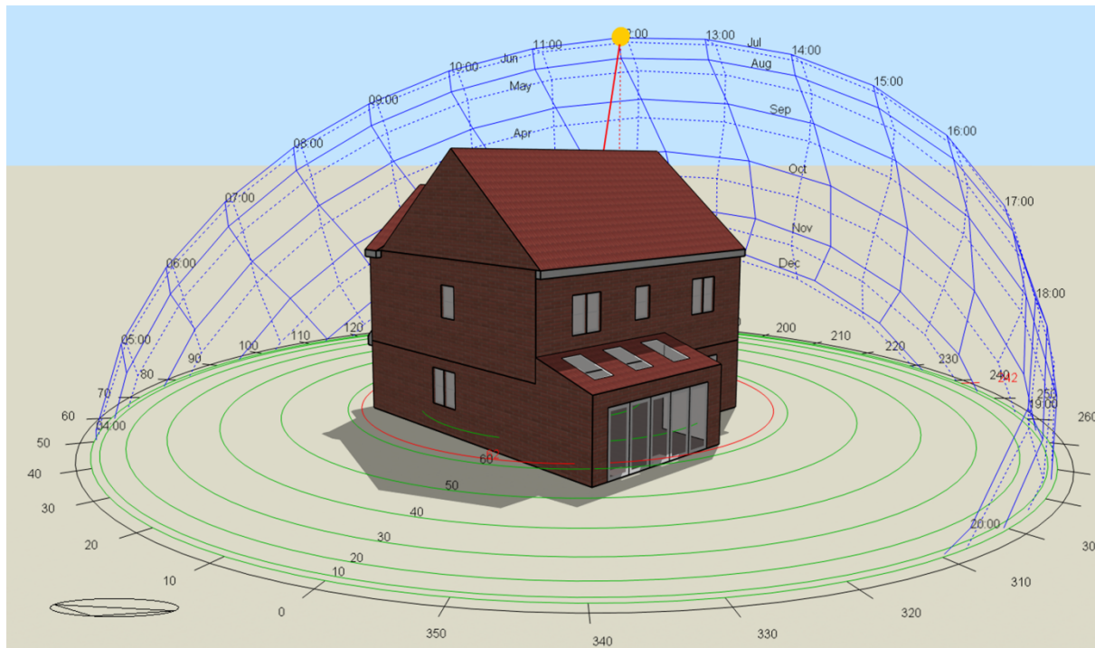
Image 7: North Perspective
