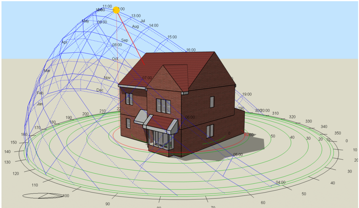
Image 4: East Perspective
