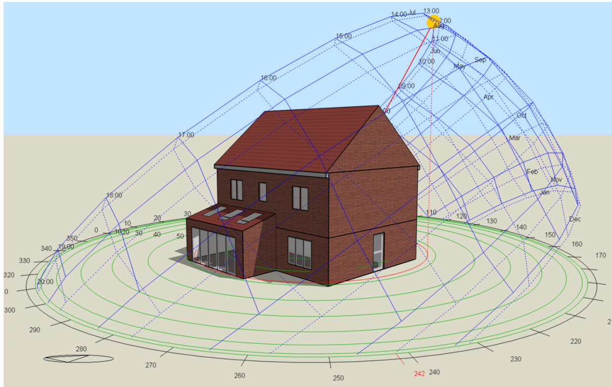
Image 6: West Perspective
