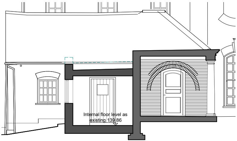
B Proposed Section West Spur Pavilion ~ BB 12003
