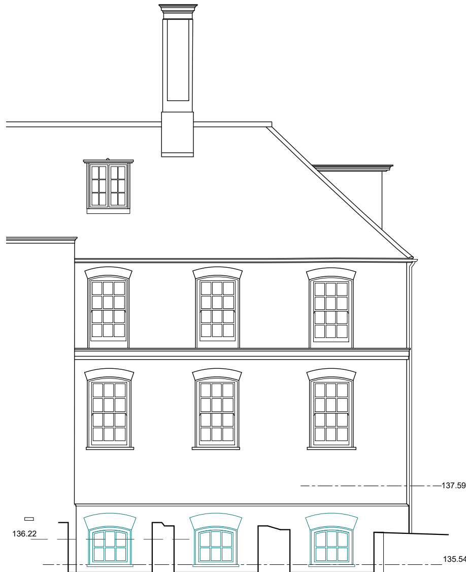
E Proposed South Elevation Stable Block ~ 12003
