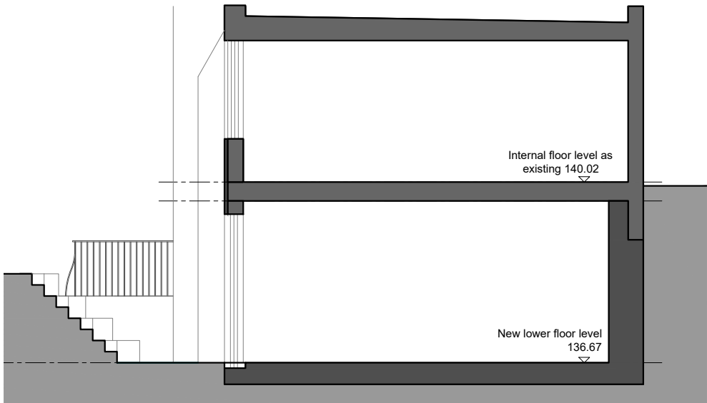
C Proposed Section West Spur Art Block ~ AA 12003
