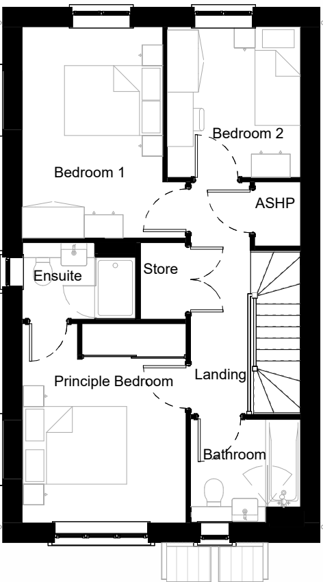
First Floor 1 : 100
