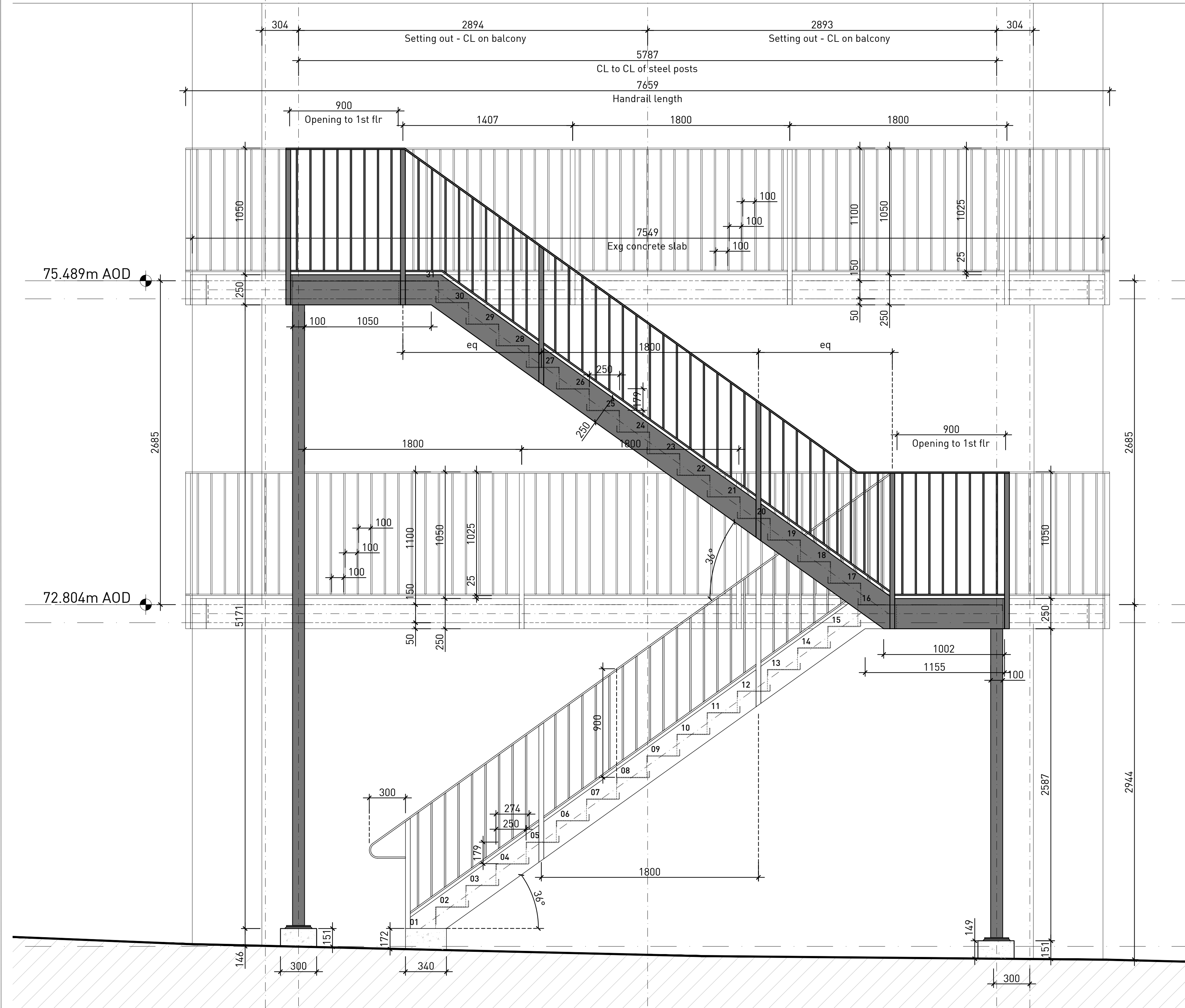
PROPOSED STAIR ELEVATIONS - STAIRCASE-5 - FRONT FACE
