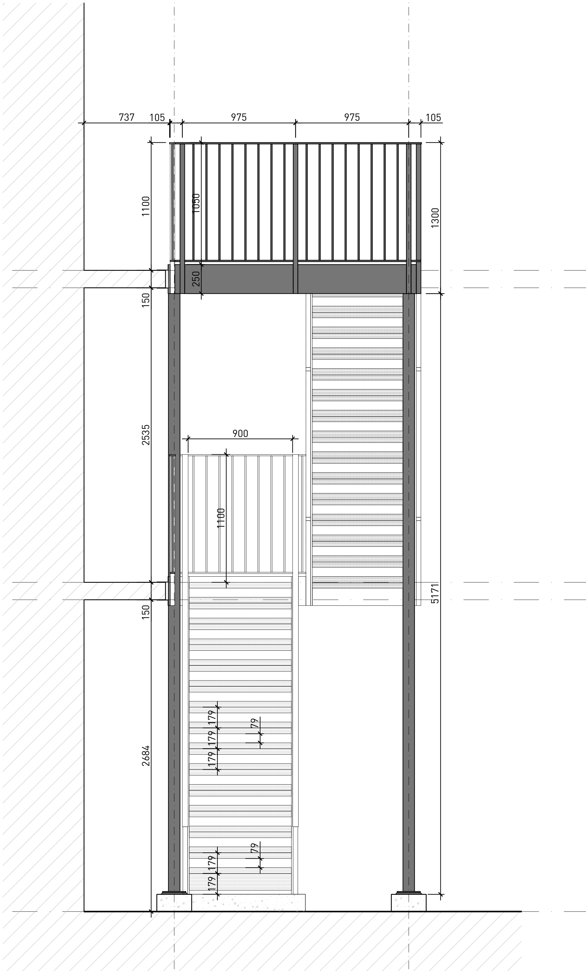
PROPOSED STAIR ELEVATION - STAIRCASE-5 - SIDE
