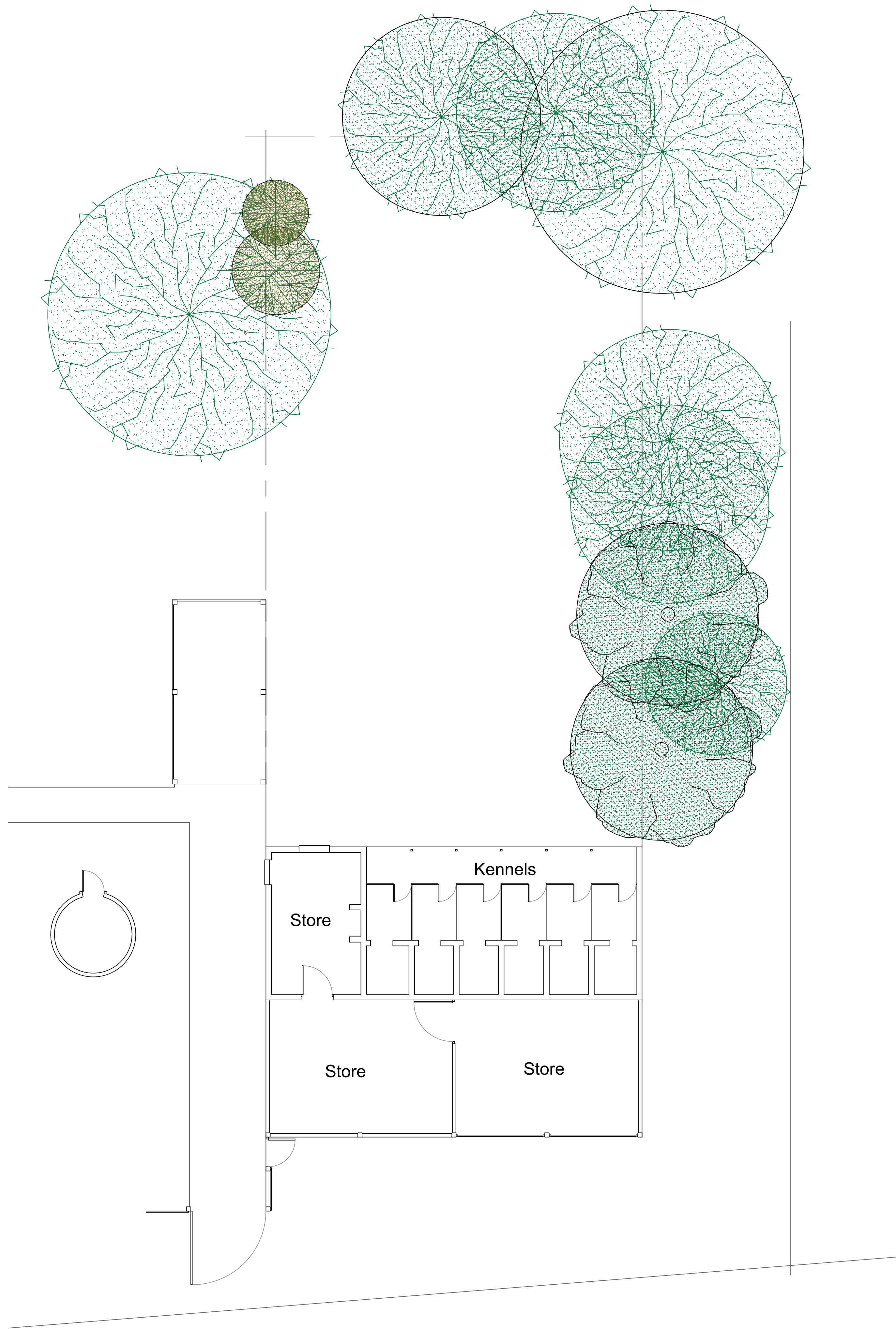
Existing Ground Floor Plan 1:100
