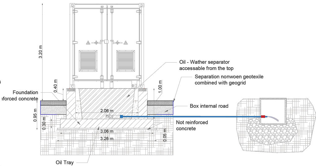
Particular of typical drainage
