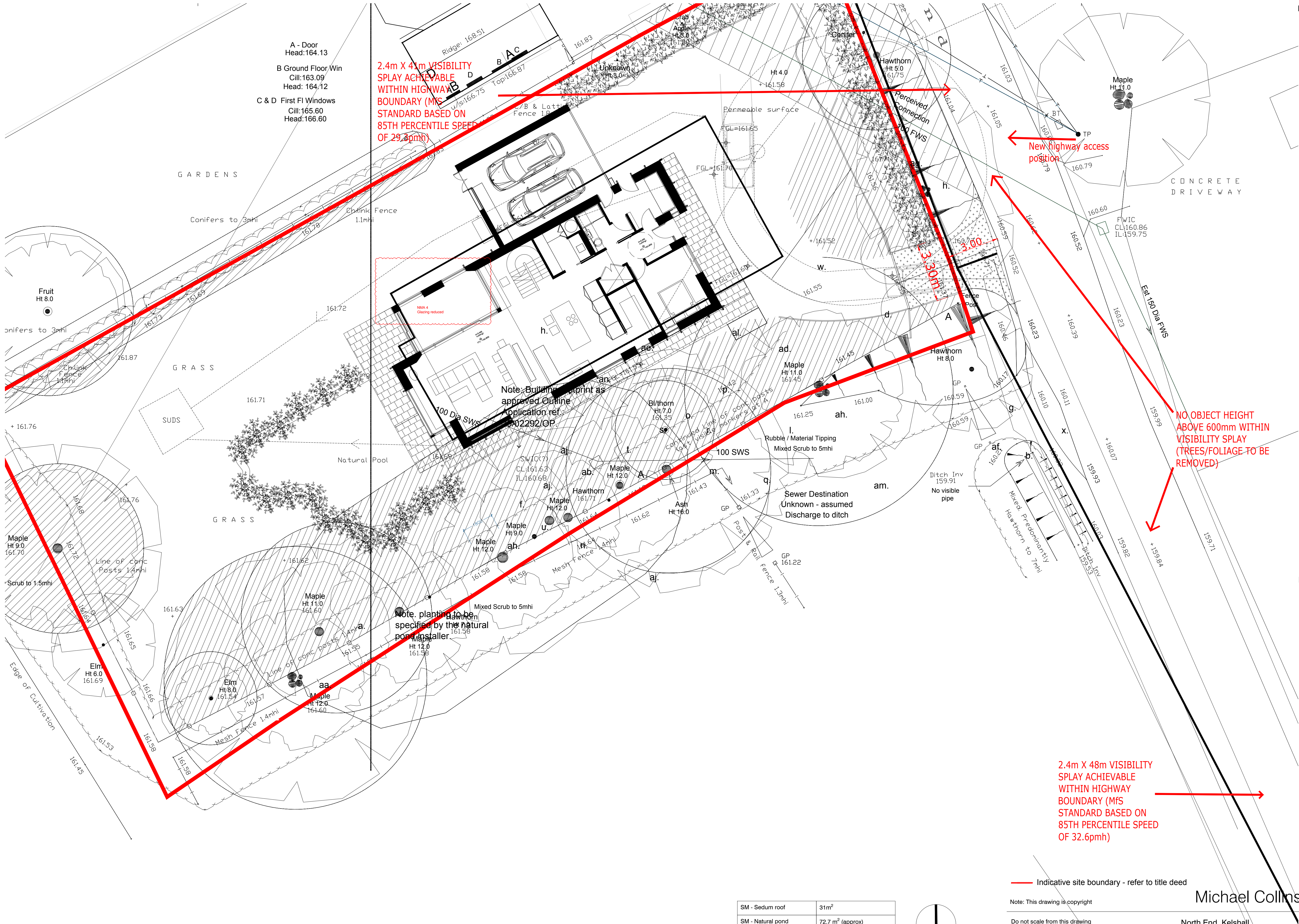
Site Plan - Ground Floor As Proposed
